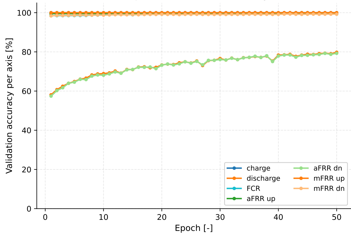
BC per-axis validation accuracy
