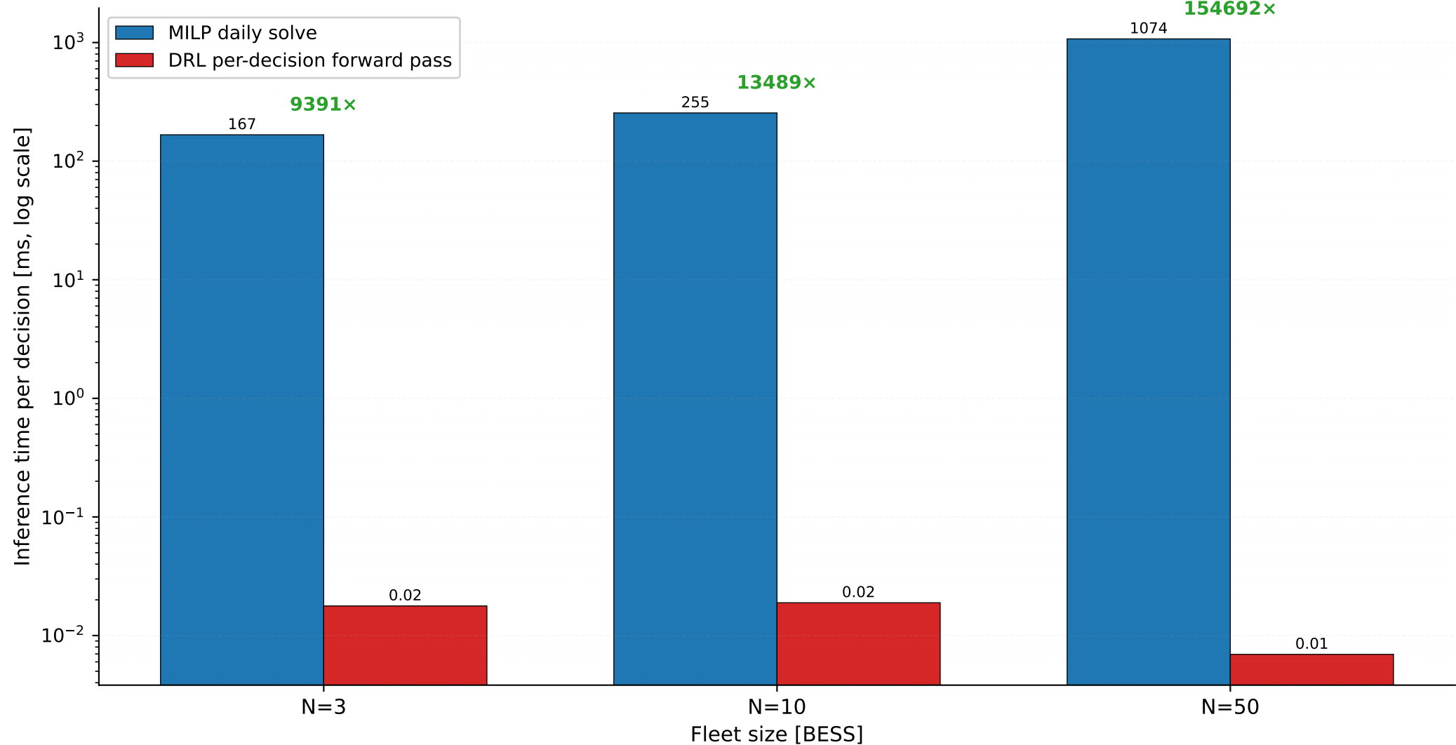
MILP vs DRL inference cost across fleet sizes
