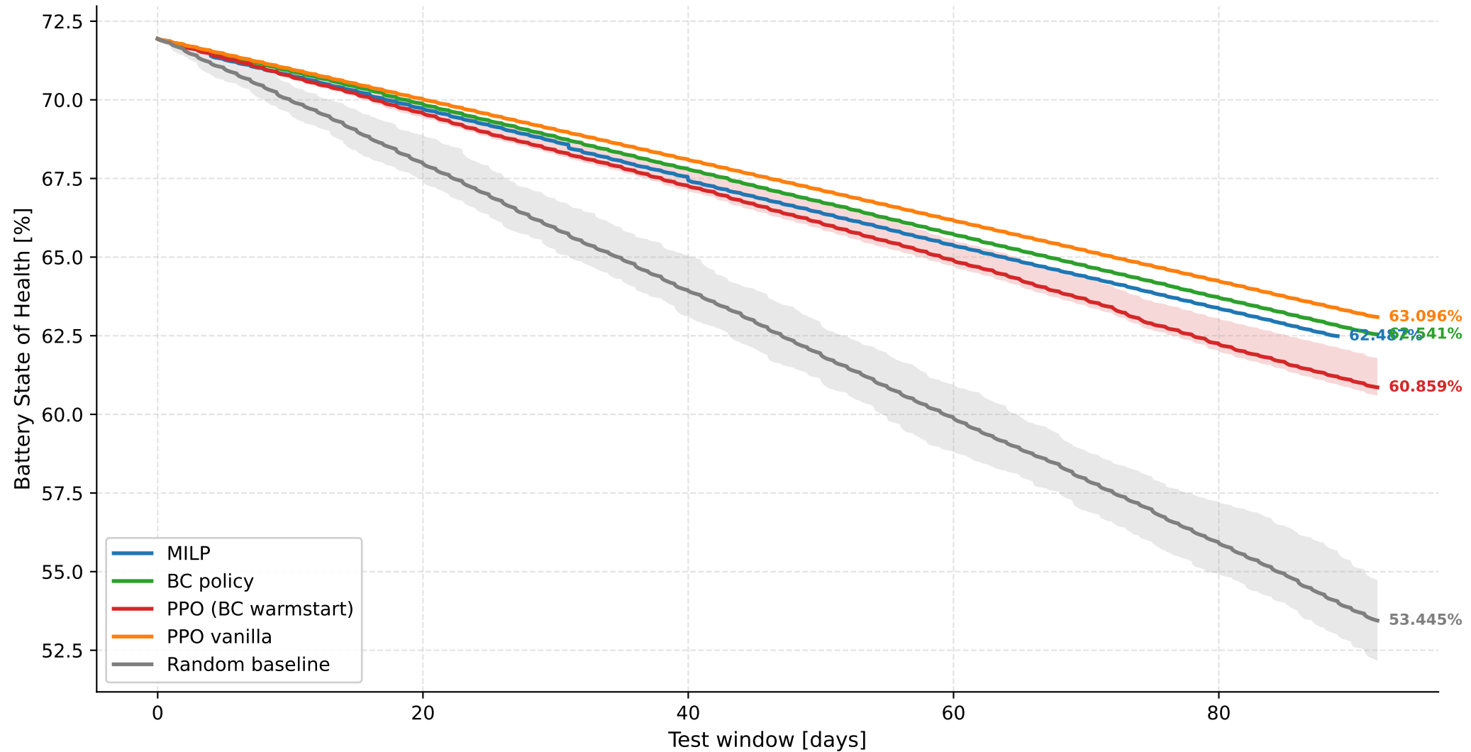
SOH degradation across policies (mean across fleet; shaded = min/max range)
