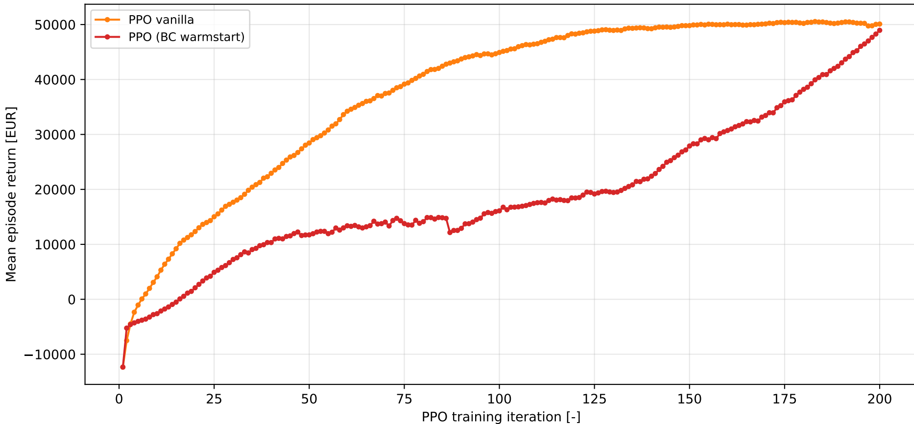
PPO learning curves on train window
