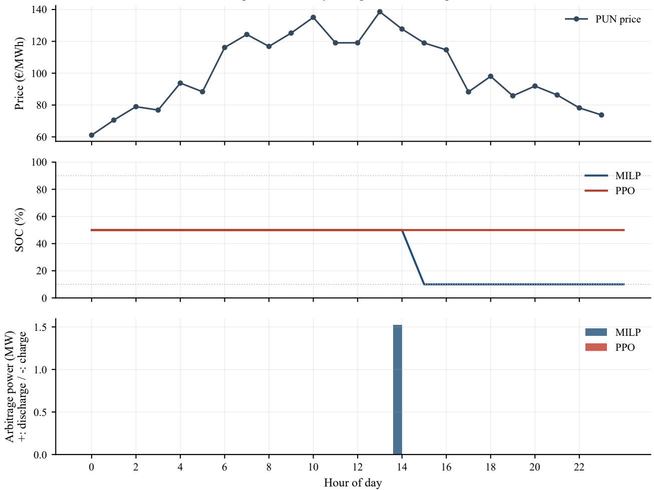
Representative day 267: price, SOC and power
