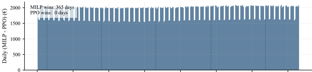
Daily profit gap and cumulative gap (ornstein-uhlenbeck)
