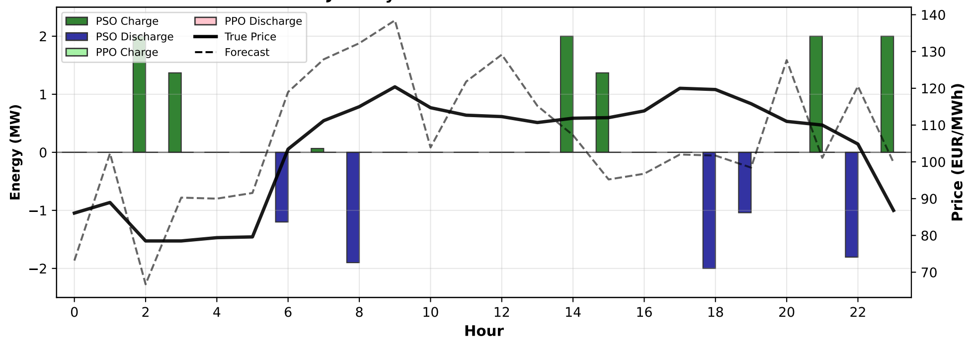
05 January 2024 - ORNSTEIN-UHLENBECK
