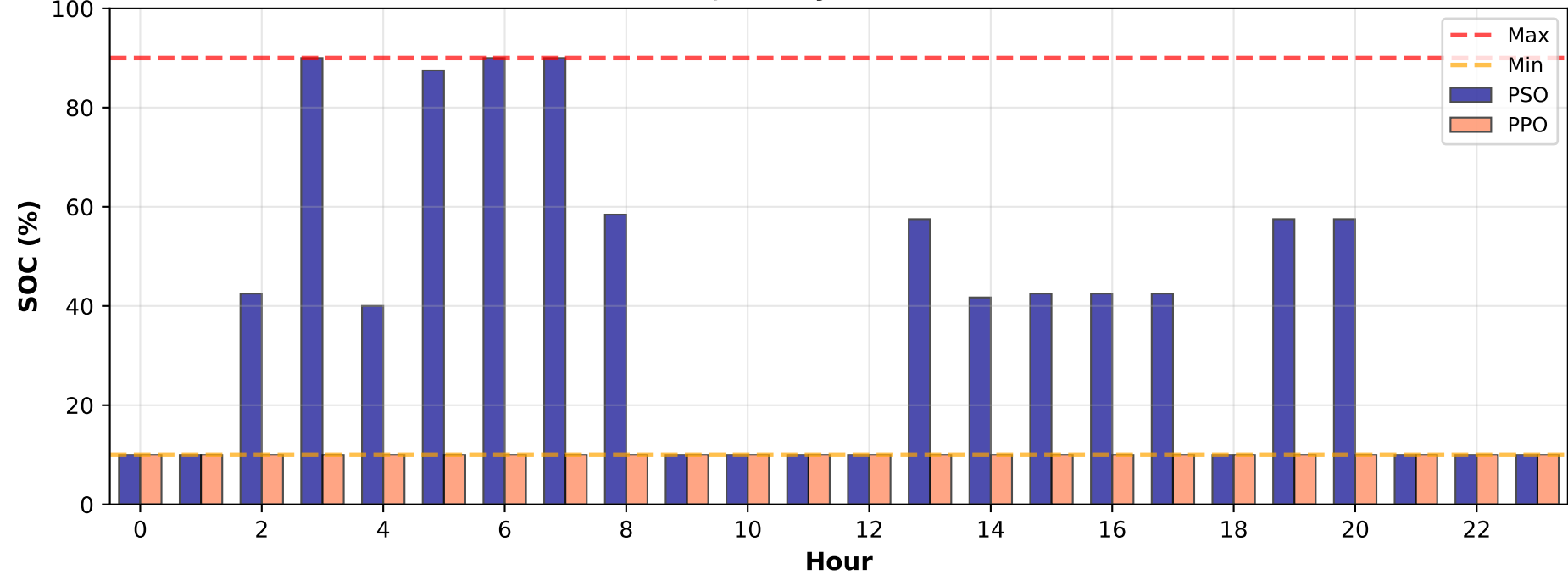
03 January 2024 - SOC
