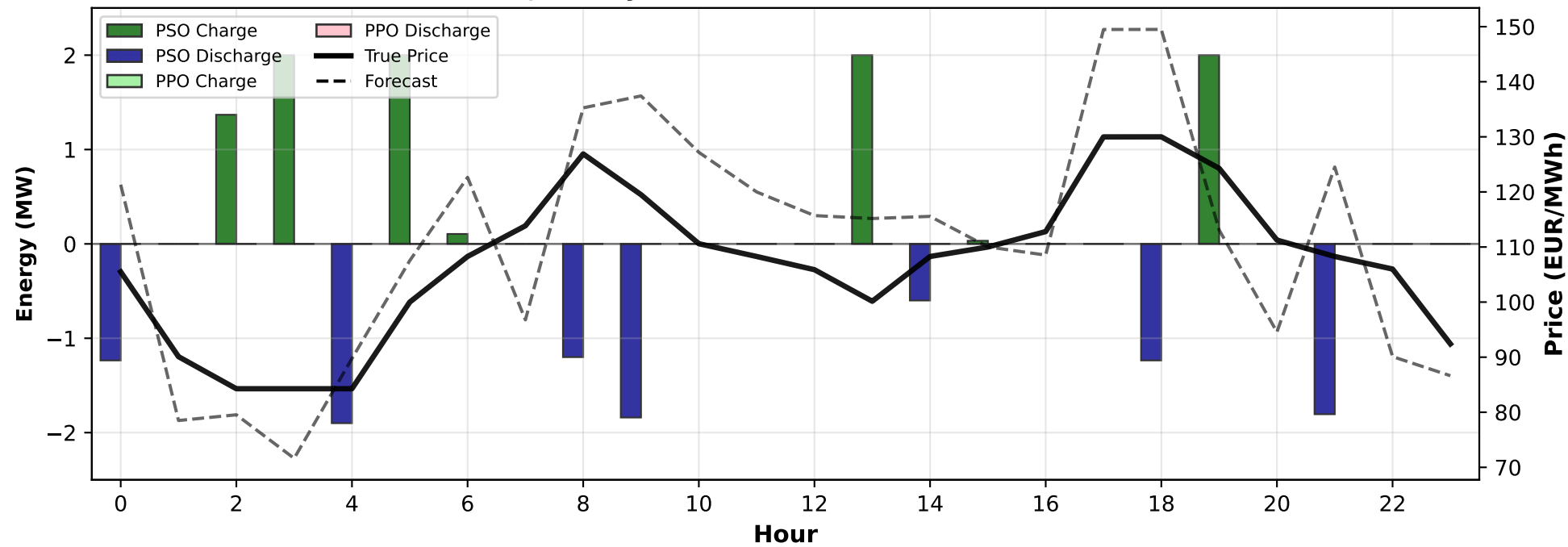
03 January 2024 - ORNSTEIN-UHLENBECK
