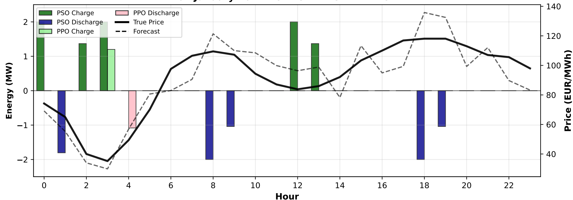
05 January 2024 - ORNSTEIN-UHLENBECK
