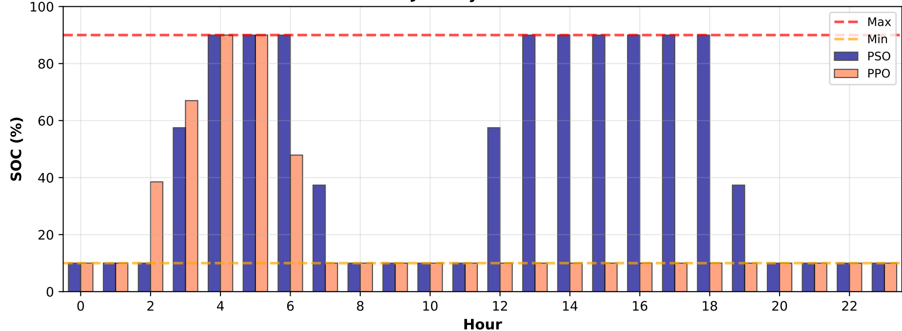
04 January 2024 - SOC
