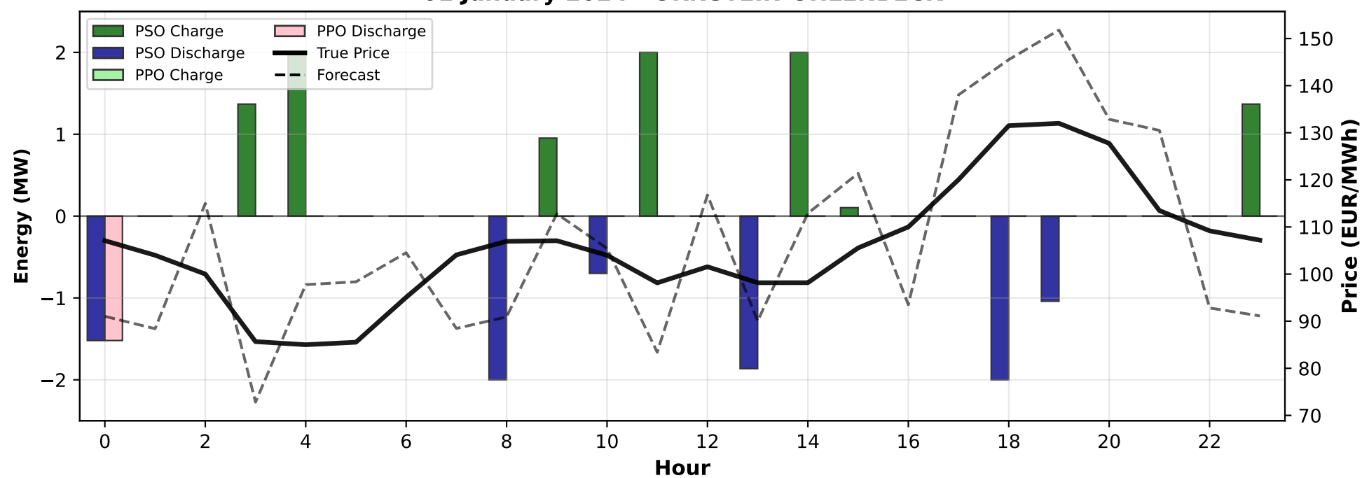
02 January 2024 - ORNSTEIN-UHLENBECK
