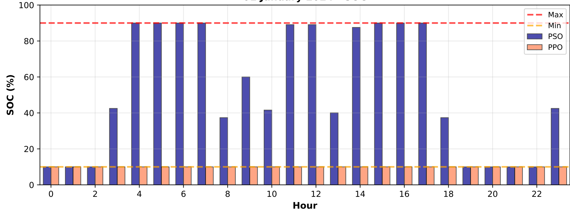
02 January 2024 - SOC
