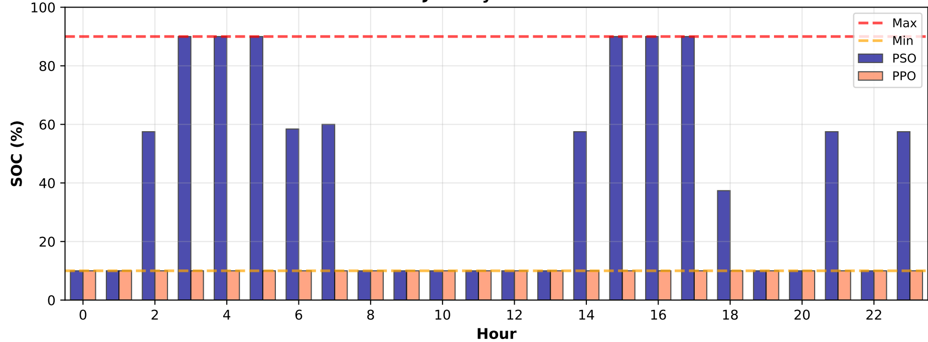
05 January 2024 - SOC
