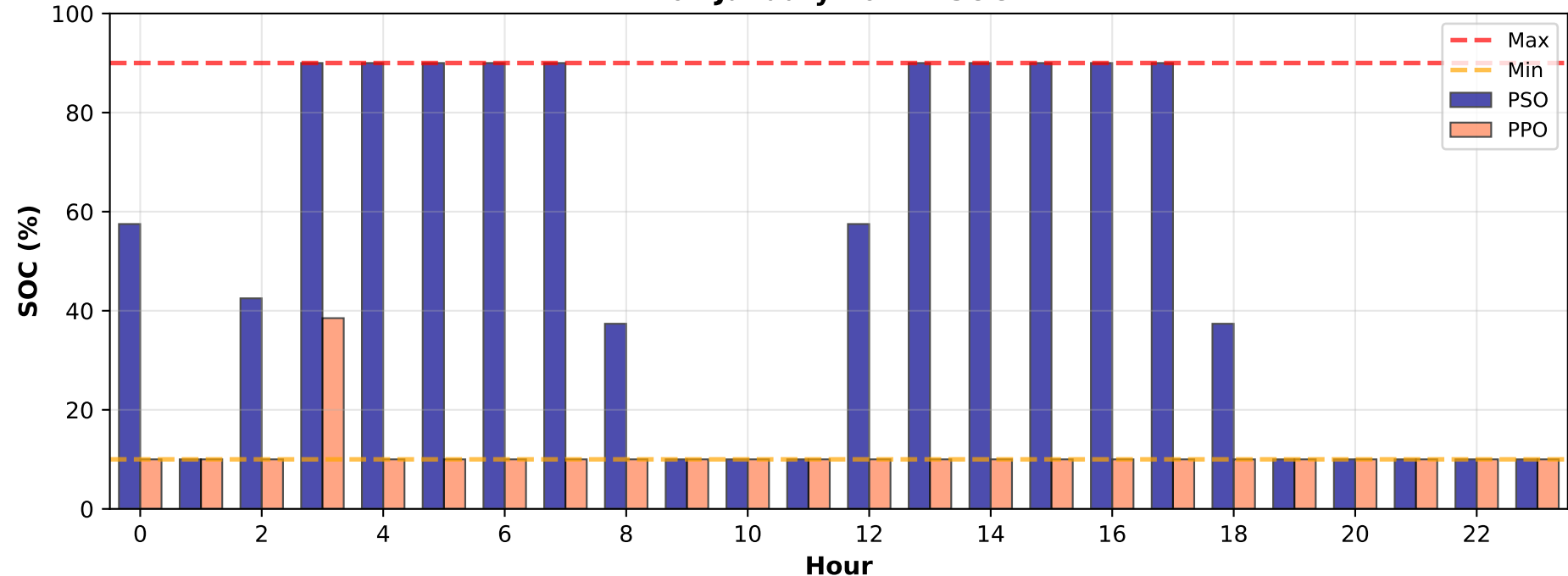
05 January 2024 - SOC
