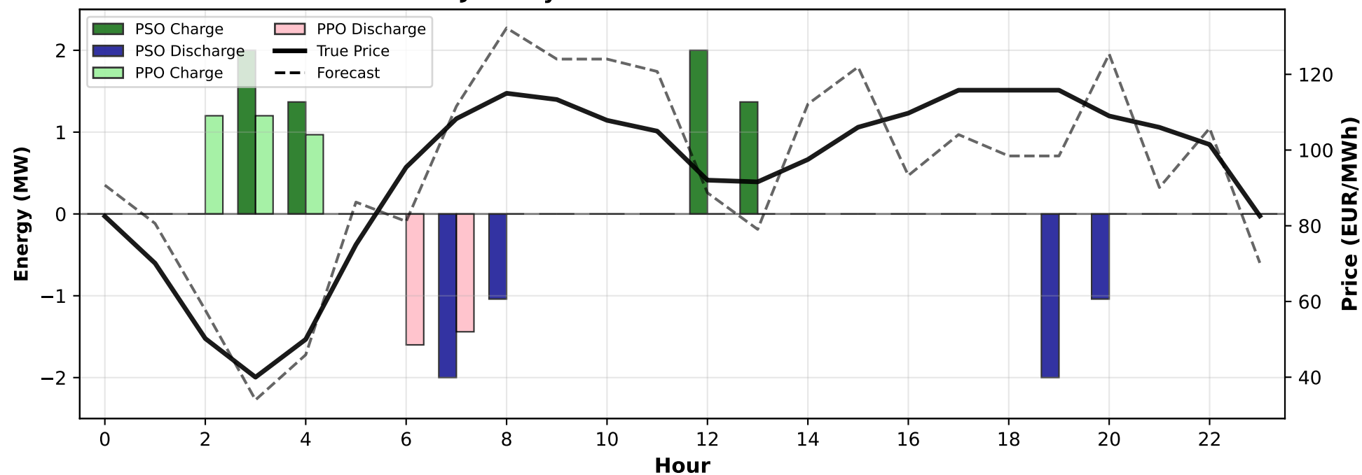
04 January 2024 - ORNSTEIN-UHLENBECK
