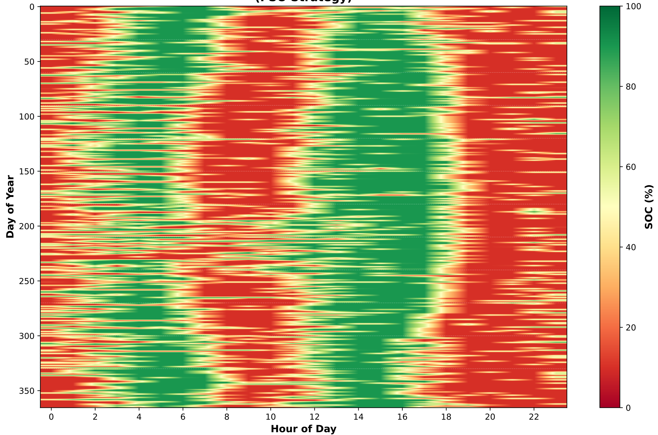
Battery State of Charge - NORMAL (PSO Strategy)
