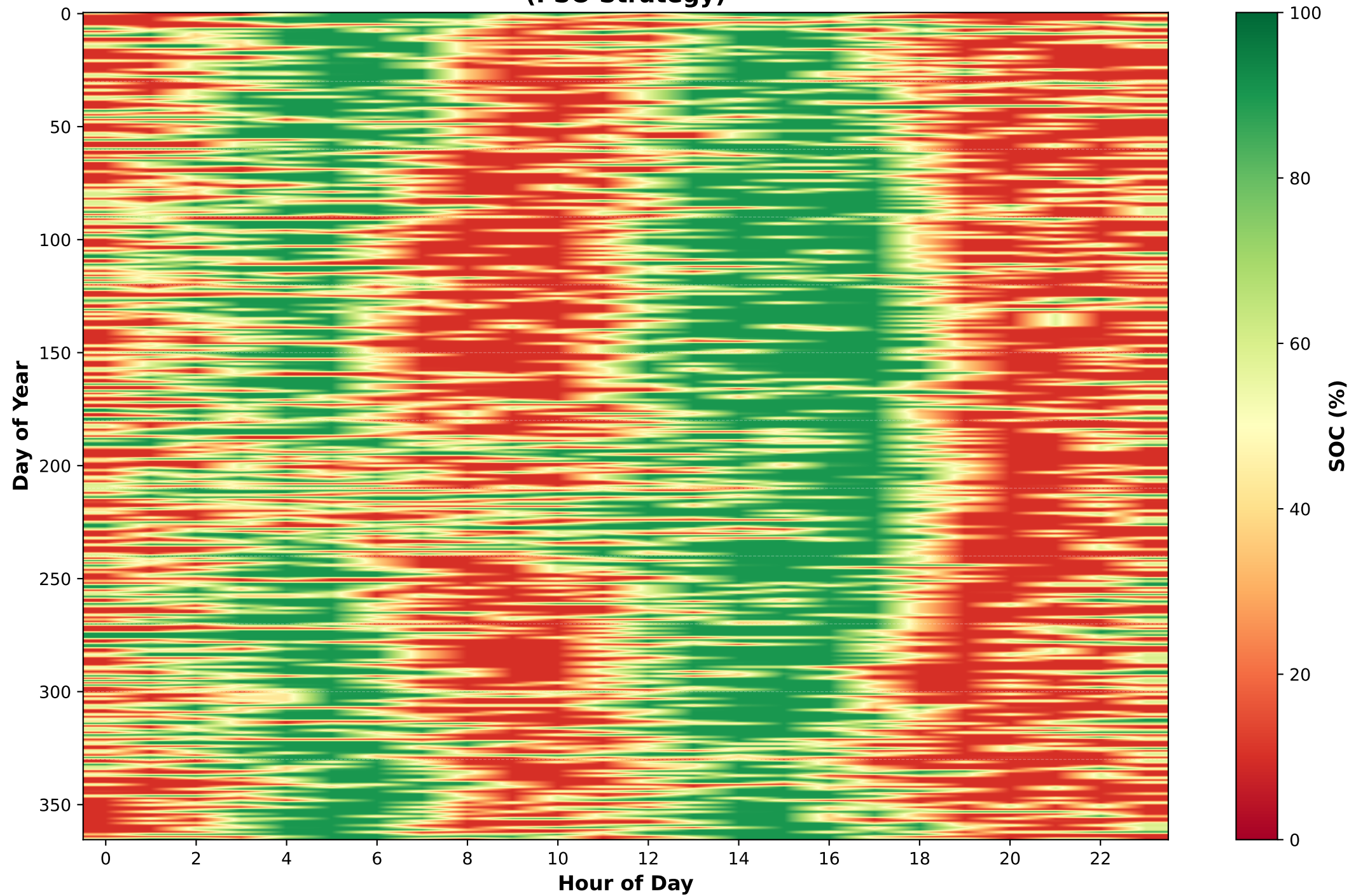
Battery State of Charge - UNIFORM (PSO Strategy)
