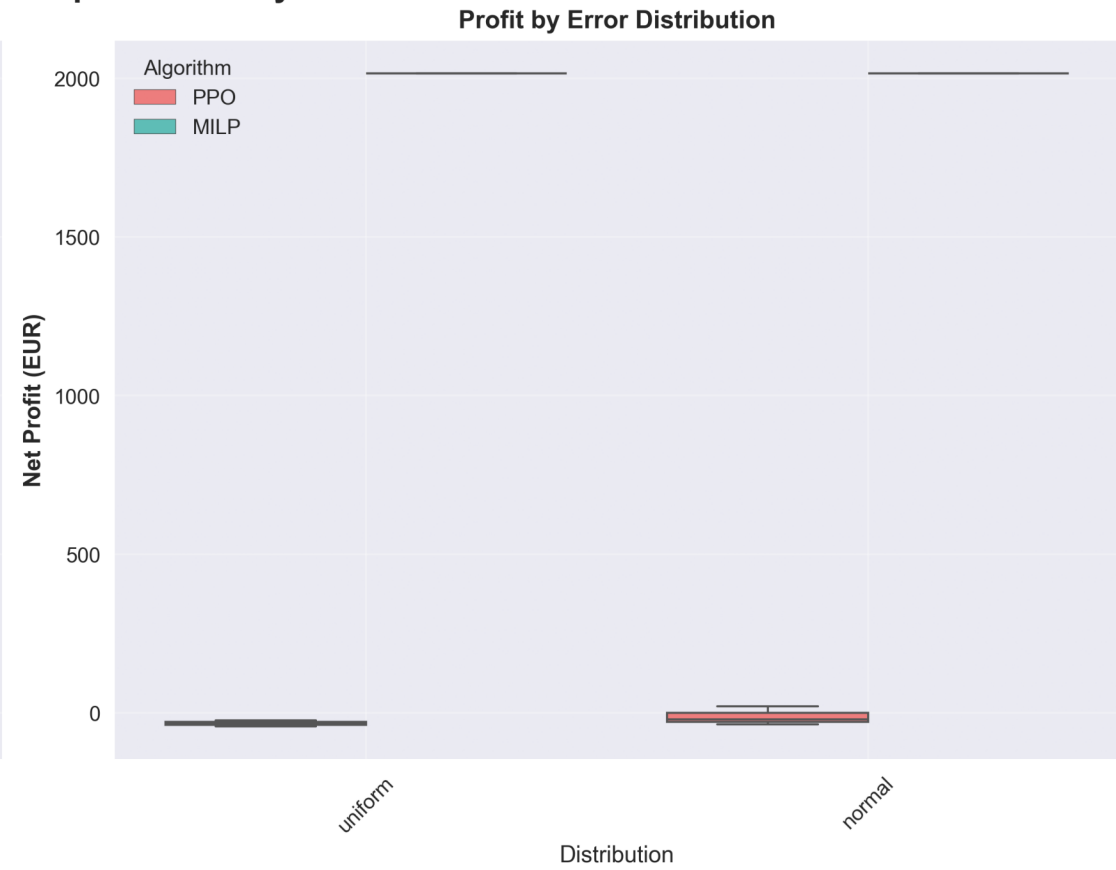
PPO vs MILP Profit Comparison Analysis
