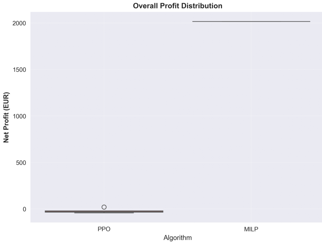
PPO vs MILP Profit Comparison Analysis
