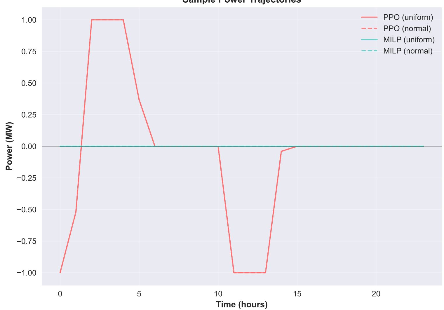
Sample Power Trajectories
