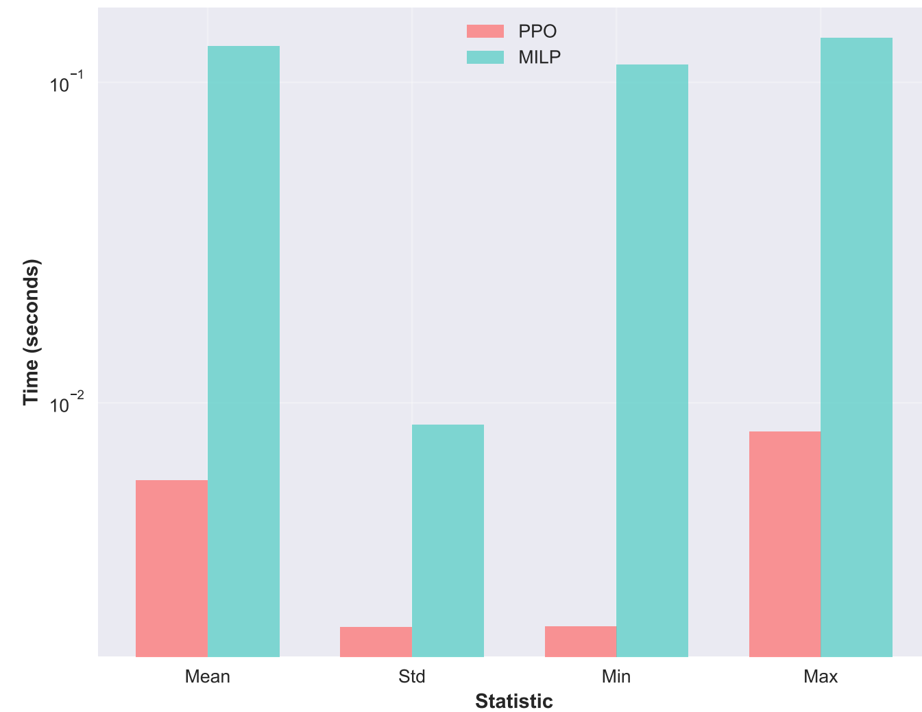
Execution Time Statistics
