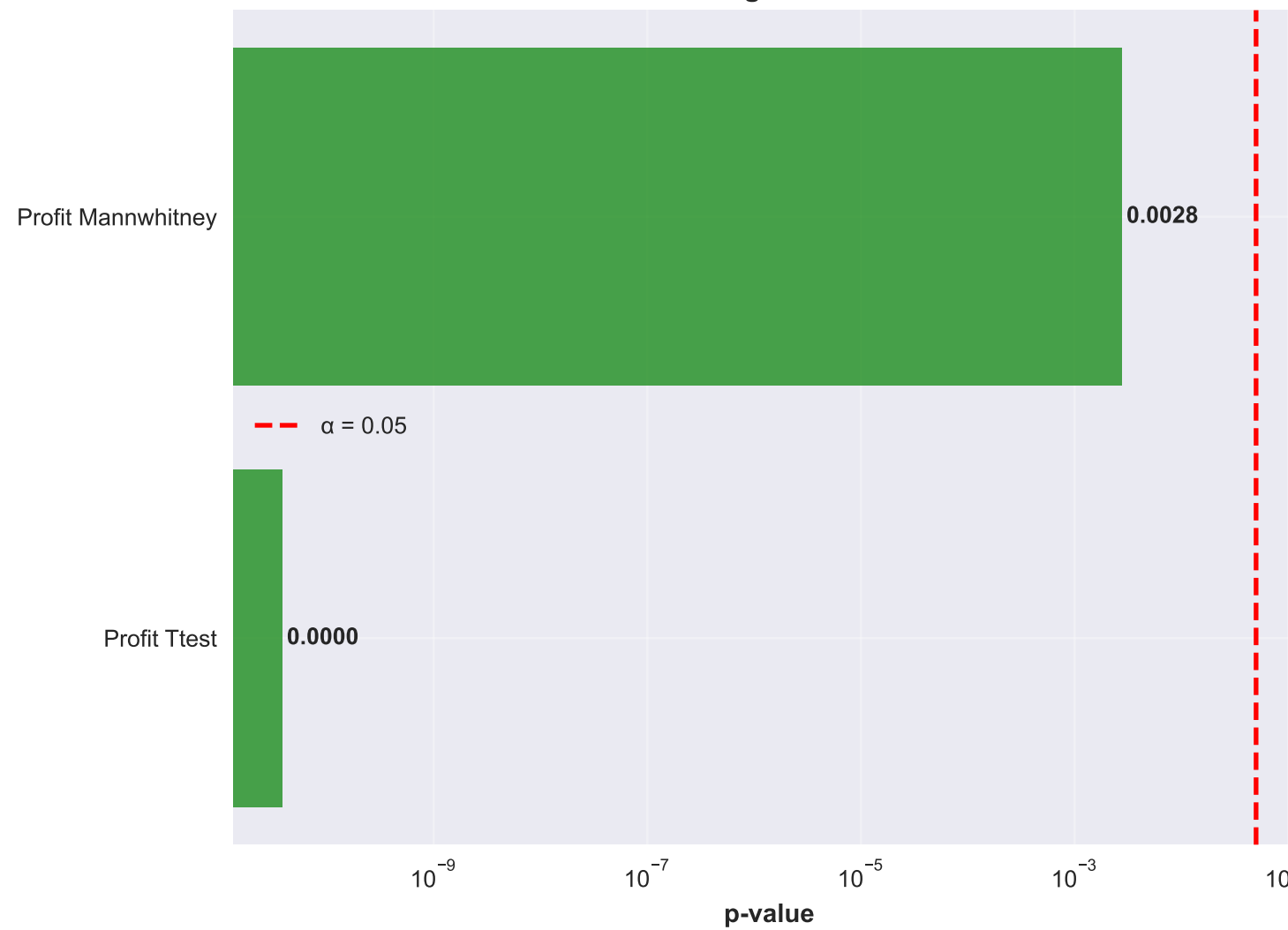
Statistical Significance Tests
