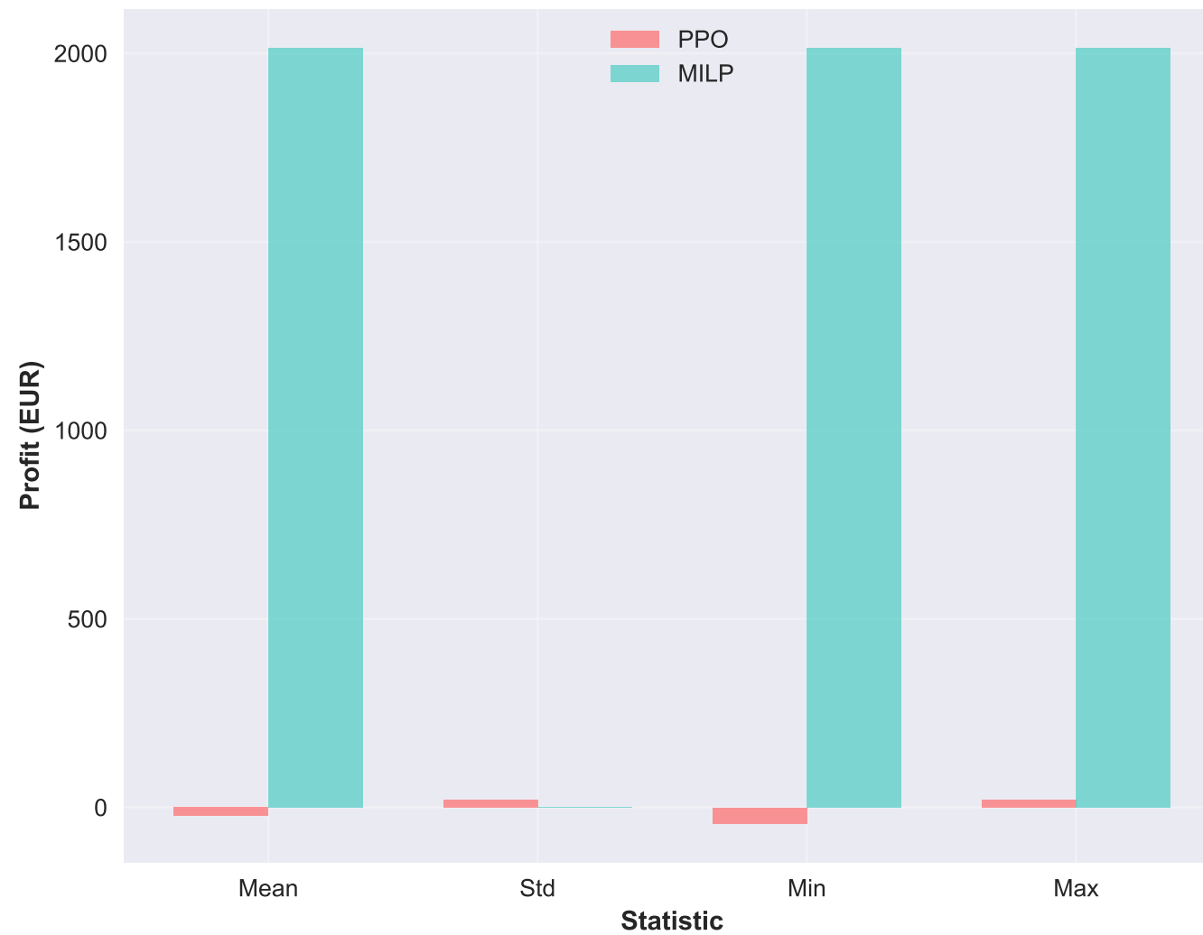
Statistical Significance Tests
