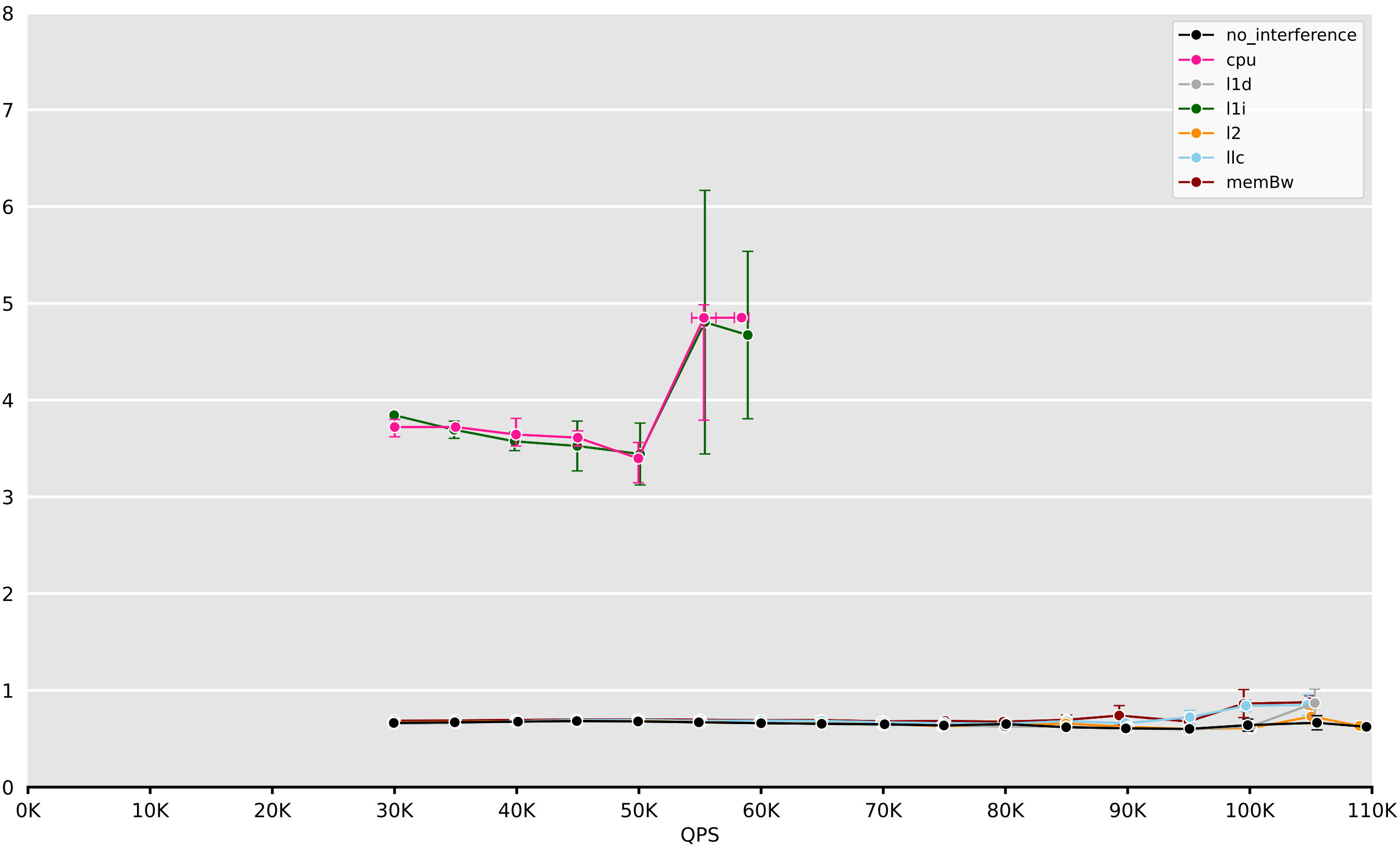
Memcached 95th Percentile Latency
