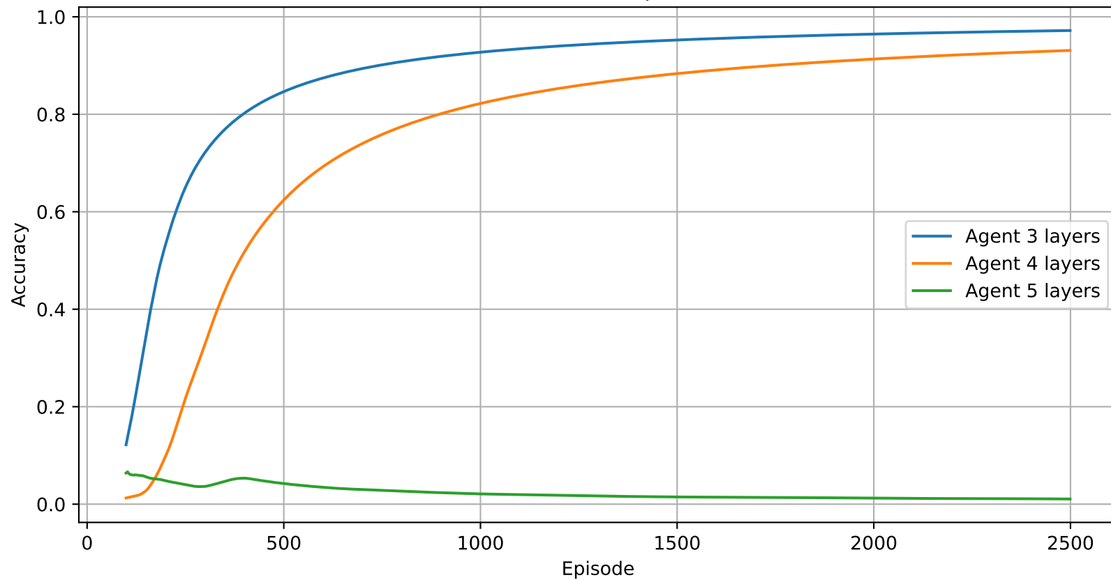
Accuracies comparison
