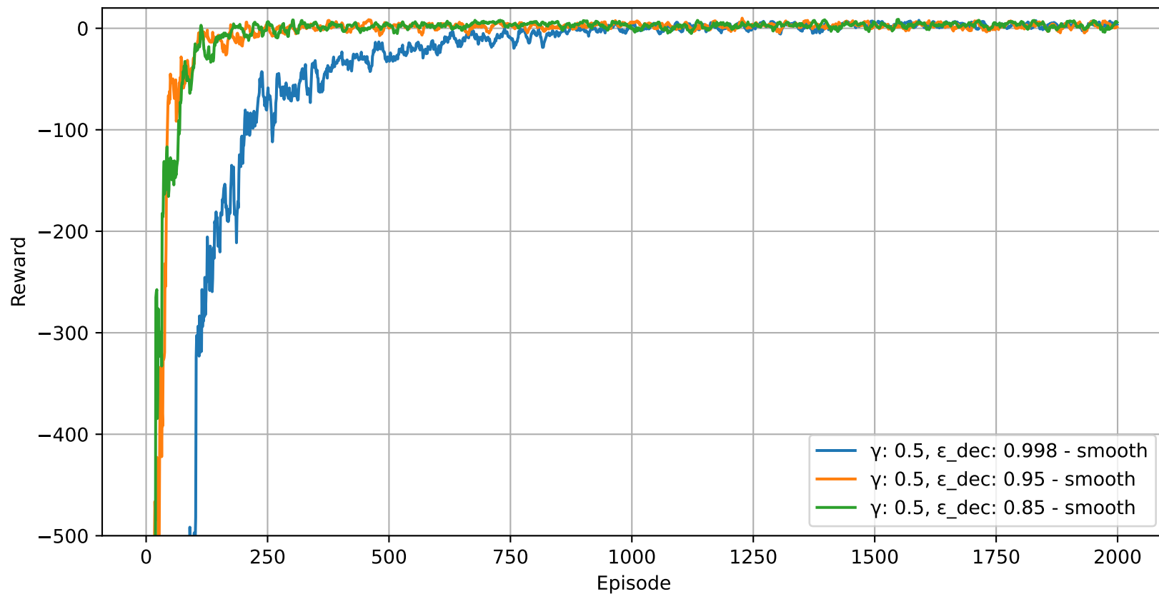
Rewards Curve for Tabular Q-Learning
