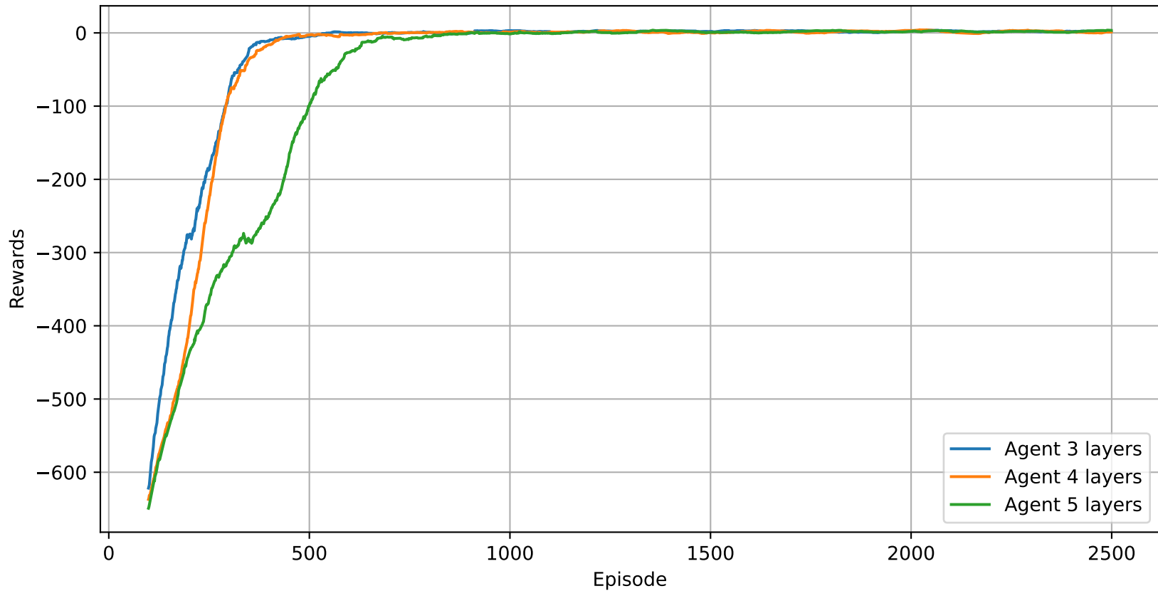
Rewards comparison
