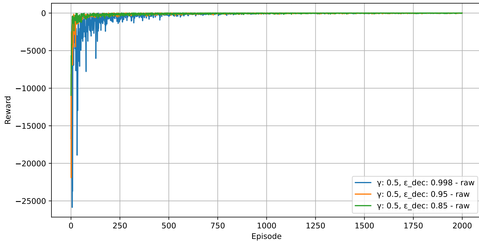
Rewards Curve for Tabular Q-Learning
