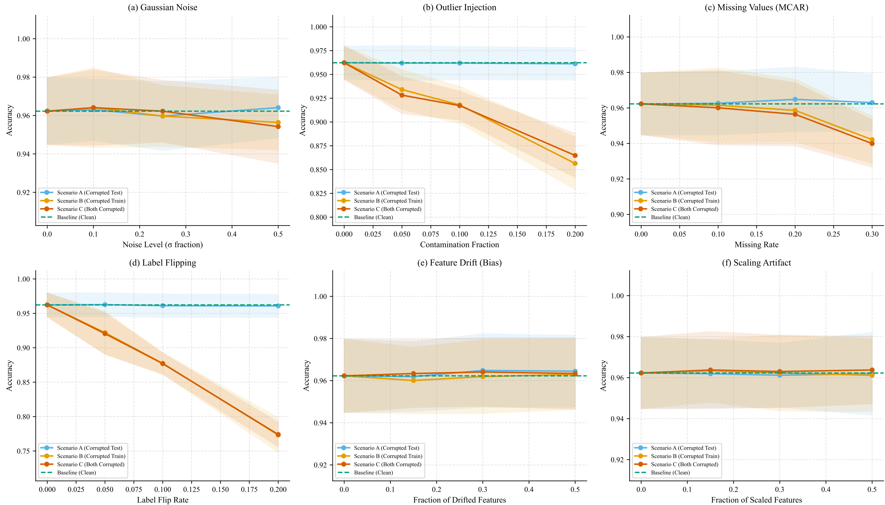
Figure 3 – Accuracy Degradation Curves by Corruption Type and Scenario
