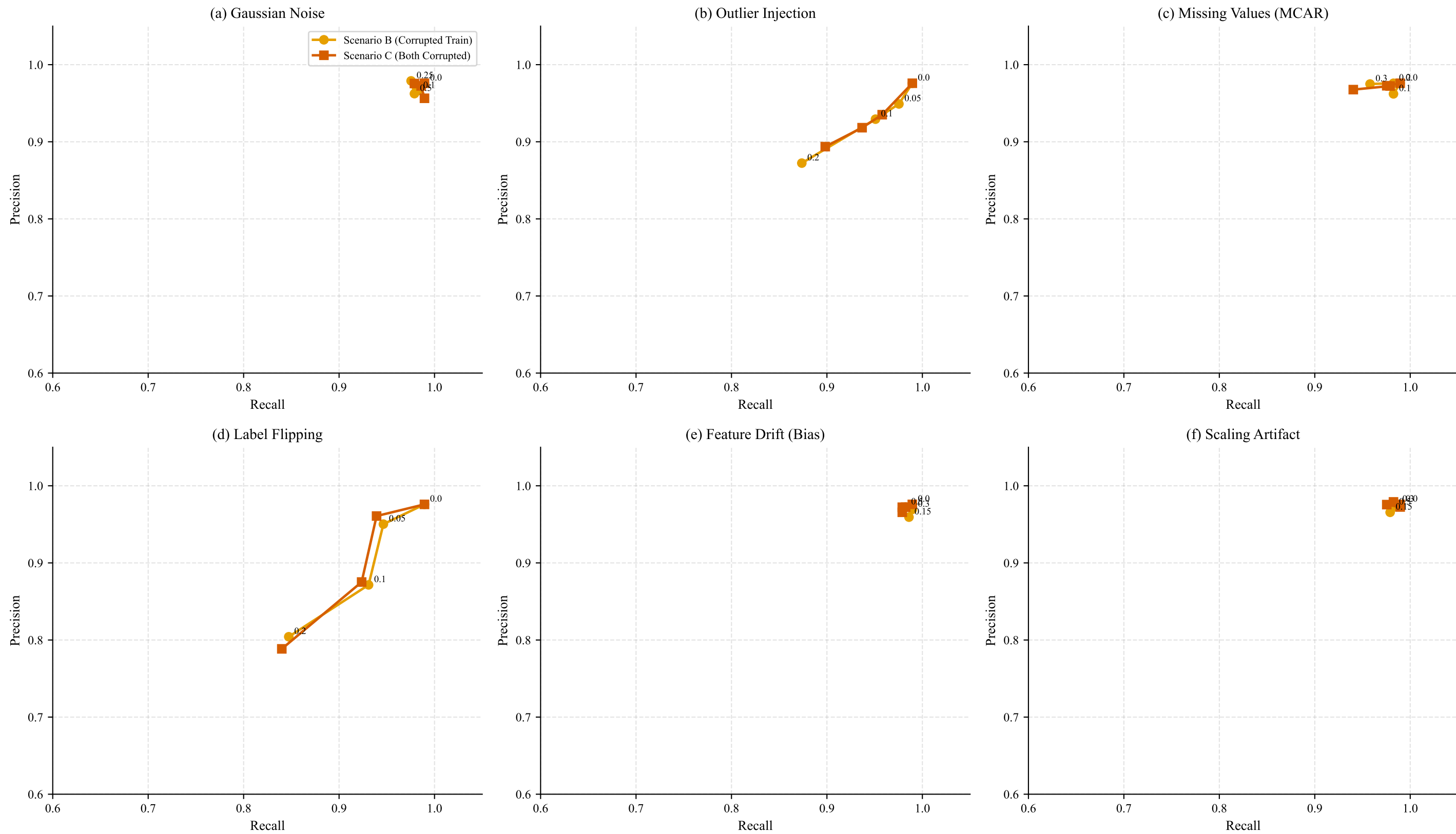
Figure 8 – Precision–Recall Trade-off (ANN + Full Features) by Corruption Level
