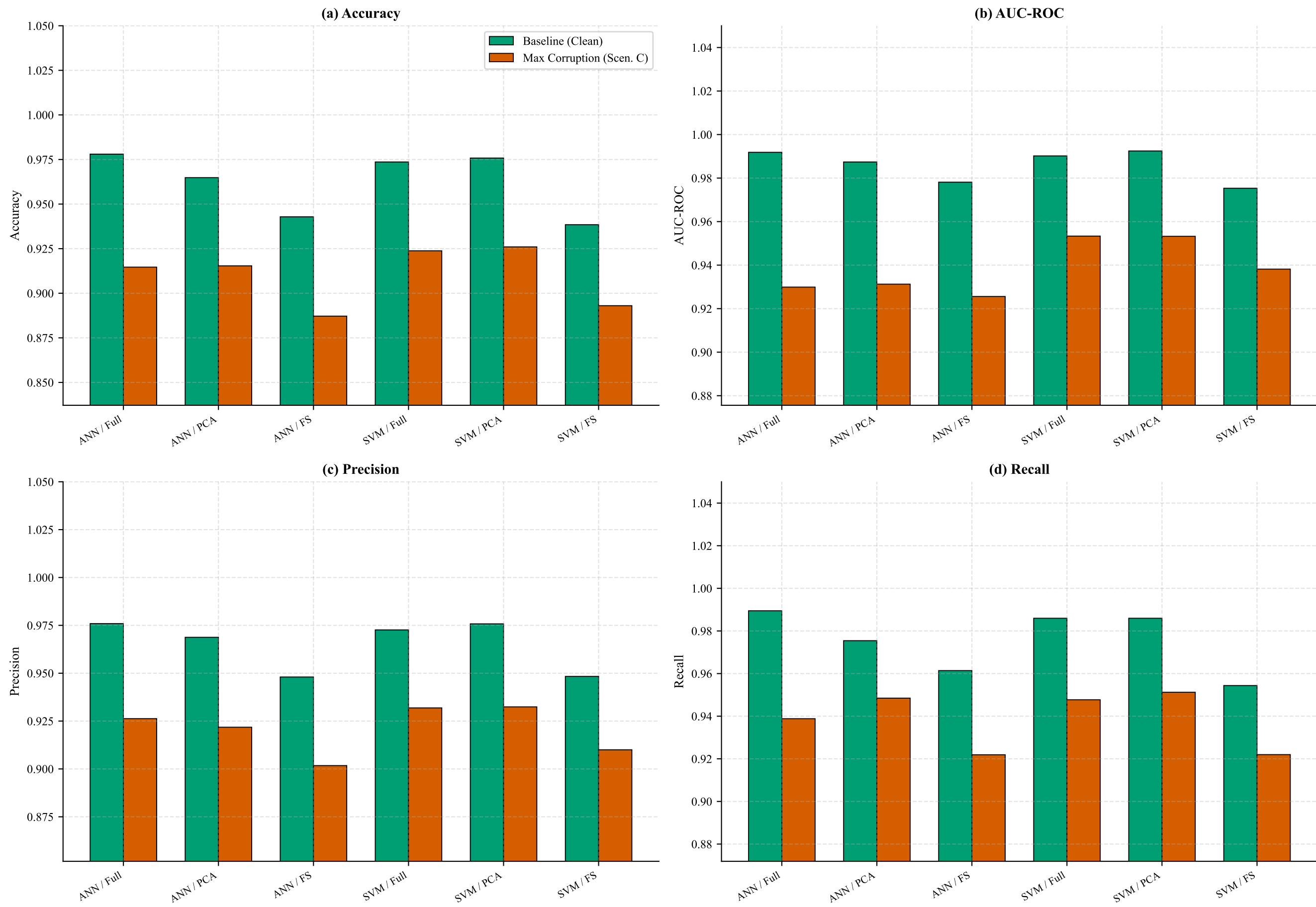
Figure 9 – Summary: Baseline vs. Worst-Case Corruption (All Metrics)
