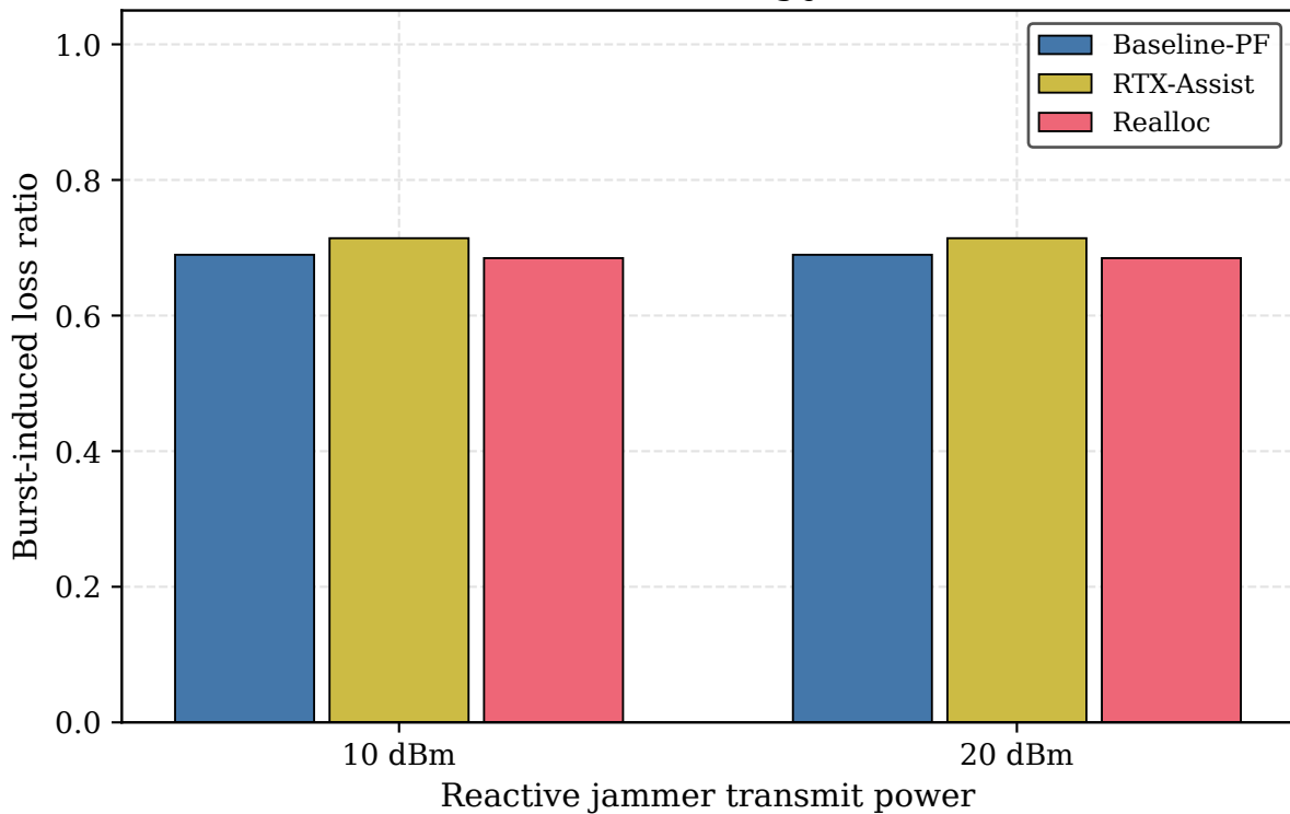
Burst-induced loss ratio (lost during jammer-ON / total losses)
