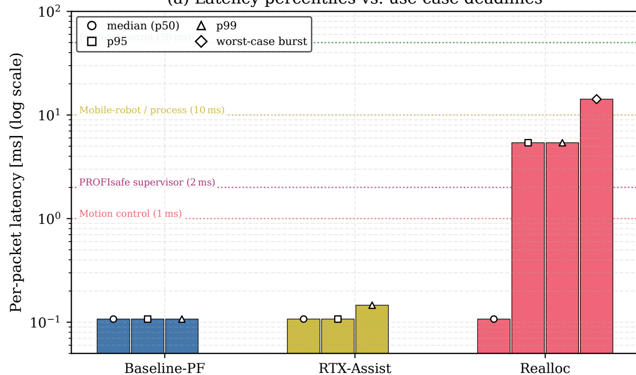
(a) Latency percentiles vs. use-case deadlines
