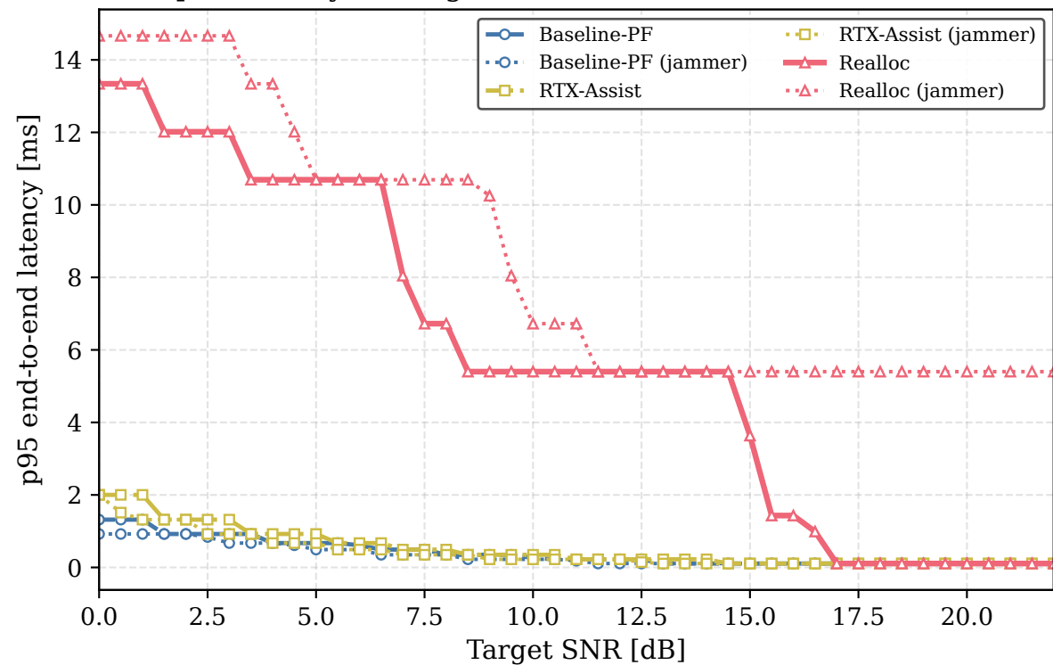
p95 latency vs. target SNR (CM8, MCS 0, 128-bit, 3 m)
