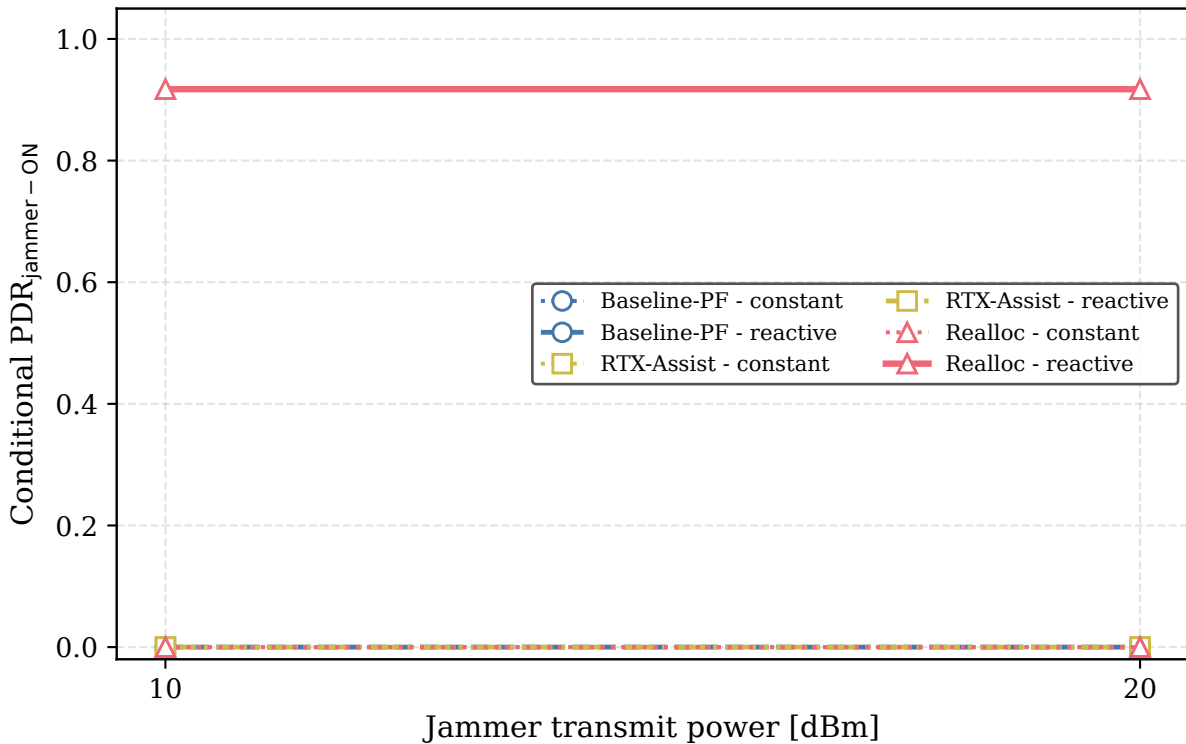
Jammer-ON PDR vs. jammer power (CM8, MCS 0, 128-bit, 3 m)
