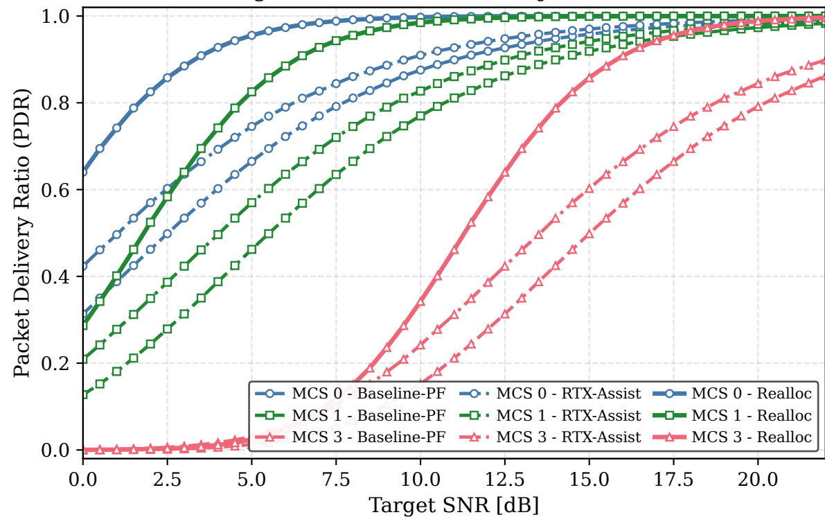
PDR vs. target SNR (CM8 NLOS, no jammer, 128-bit, 3 m)
