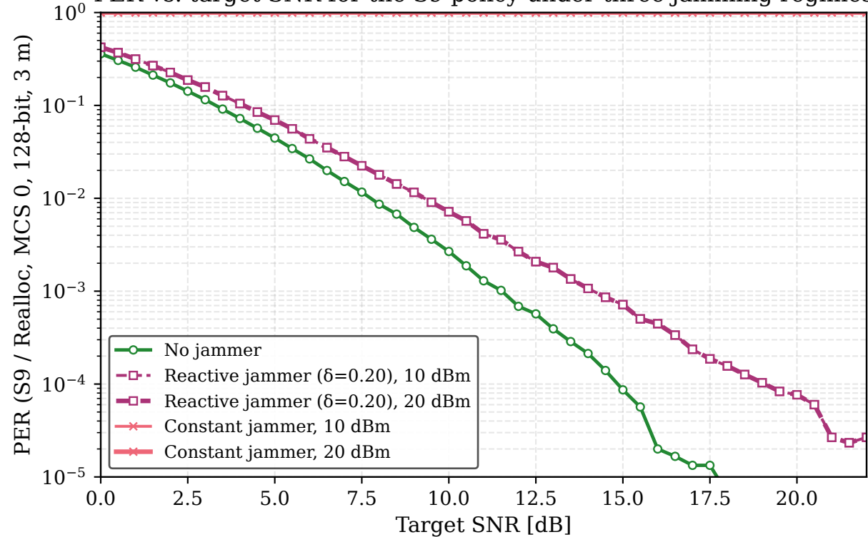
PER vs. target SNR for the S9 policy under three jamming regimes
