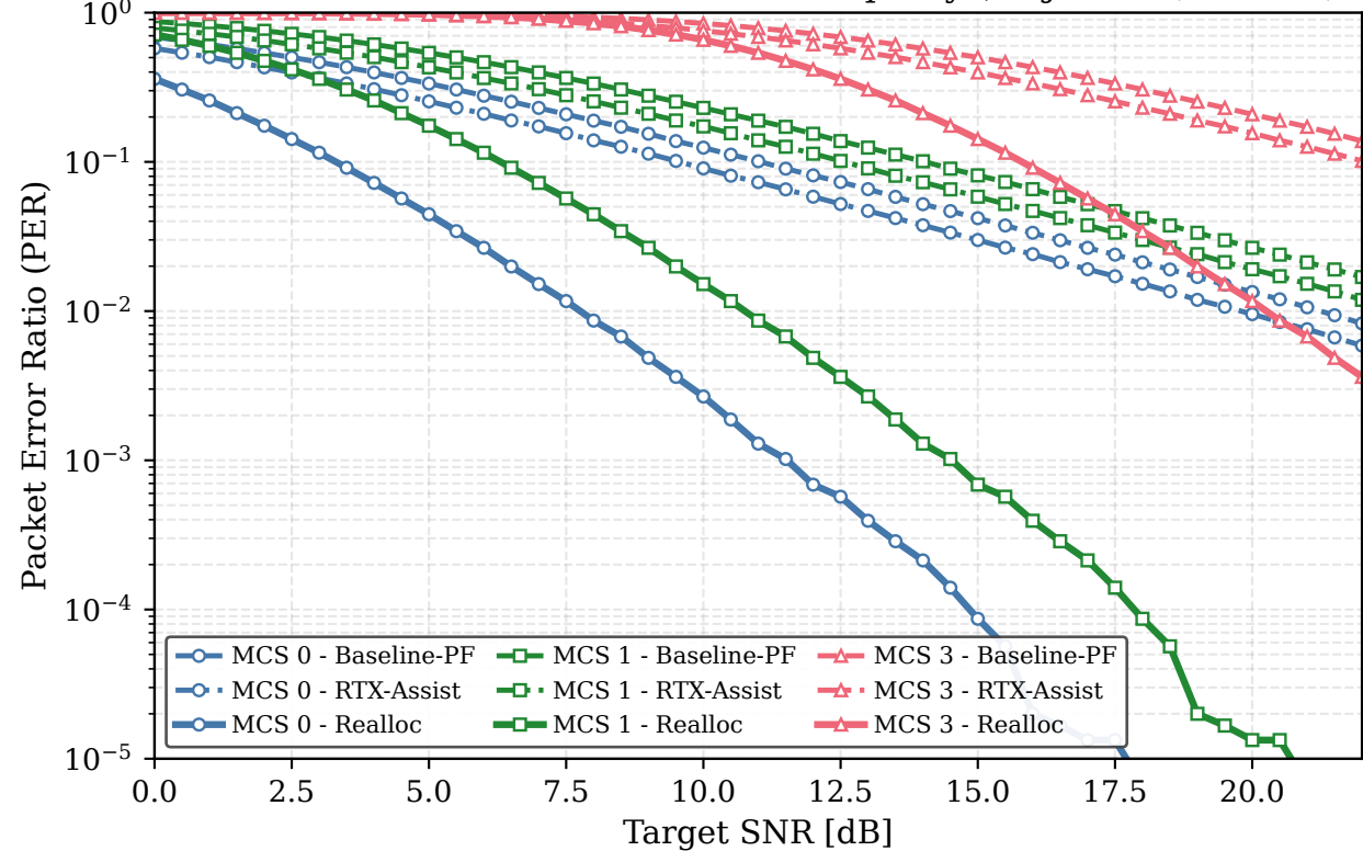
PER waterfall on the CM8 industrial NLOS proxy (no jammer, 128-bit, 3 m)
