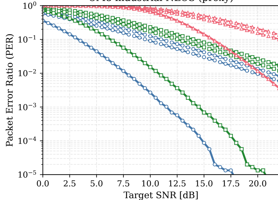
CM8 industrial NLOS (proxy)
