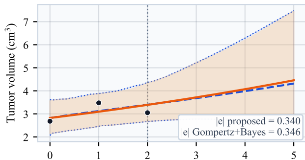
(a) Comparison for patient 100111
