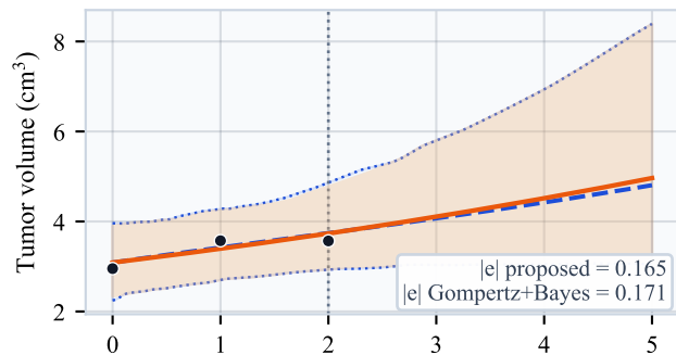
(b) Comparison for patient 100056
