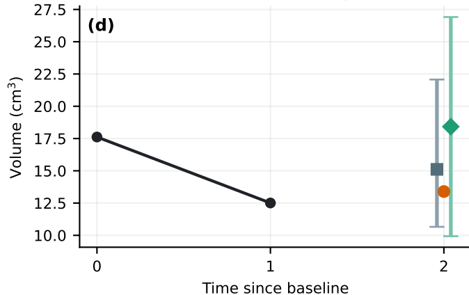
Case 4: decreasing
