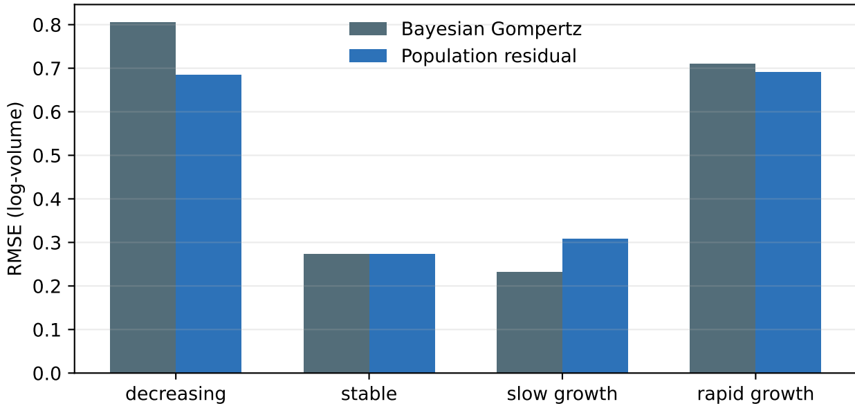
Prediction error by trajectory class
