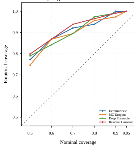
D. Subgroup PICP
