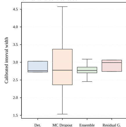
C. Interval width distribution
