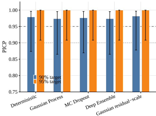
A. m = 4 calibrated PICP with Wilson CI
