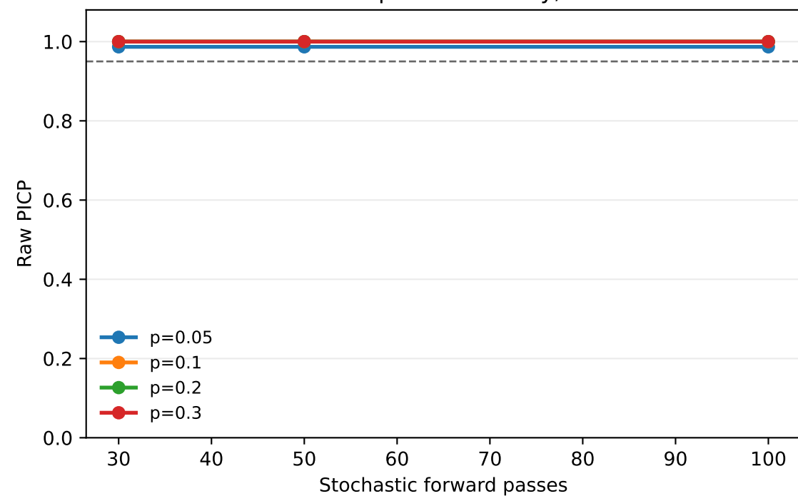
D. MC Dropout sensitivity, m=4
