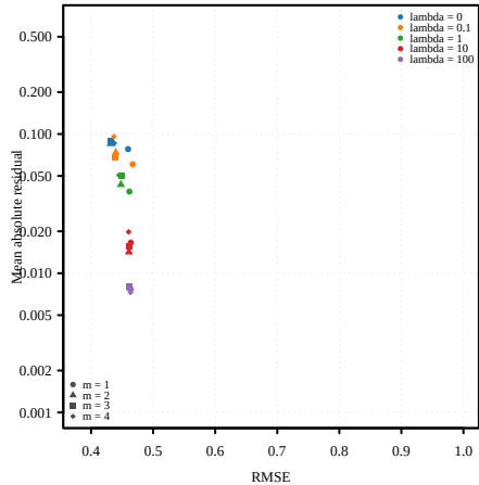
C. Accuracy-residual trade-off
