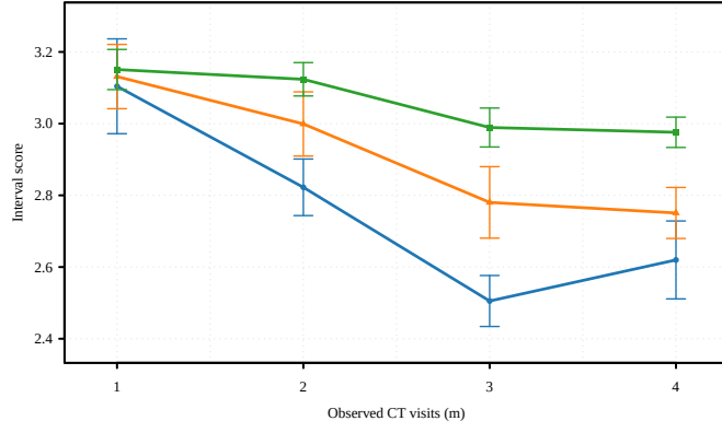
D. Gompertz-style residual
