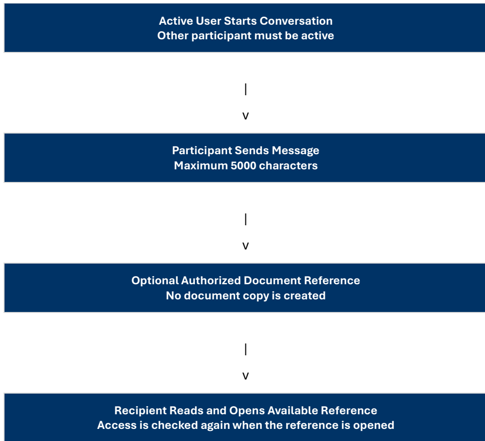
Figure 5 Participant only Messages flow
