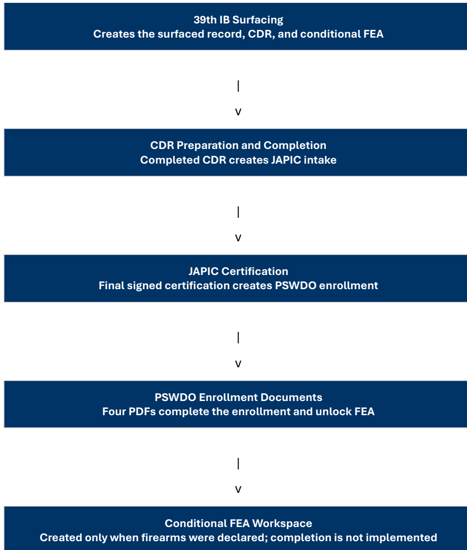
Figure 1 Former Rebel inter agency document pipeline
