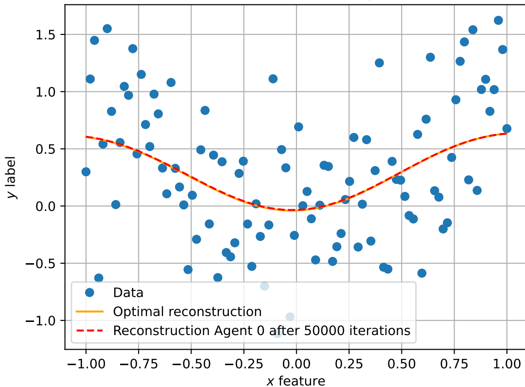
Reconstruction of the function with DGD compared to the exact solution
