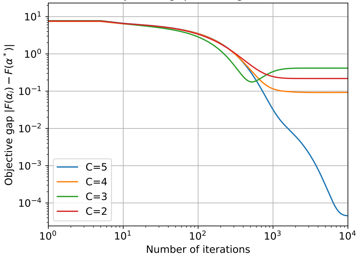
FedAVG : Objective gap convergence, E=5, B=20
