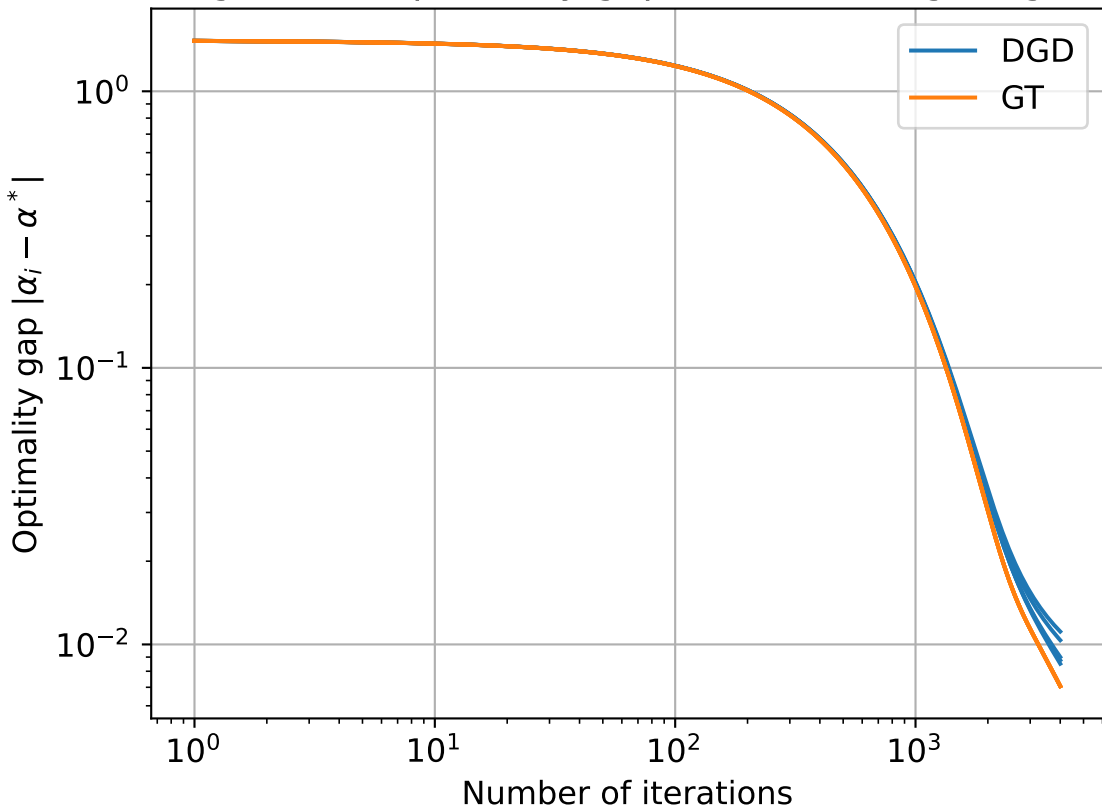
Convergence of optimality gap on Kernel ridge regression
