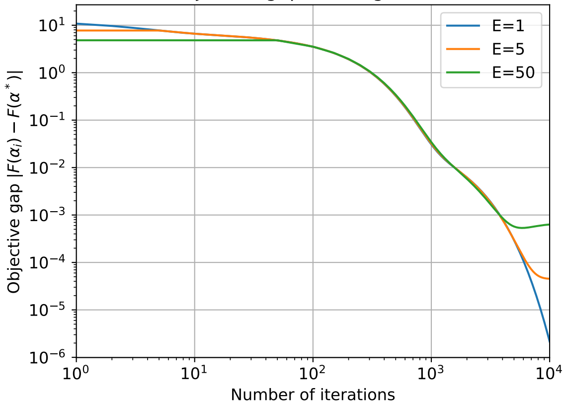
FedAVG : Objective gap convergence, B=20, C=5
