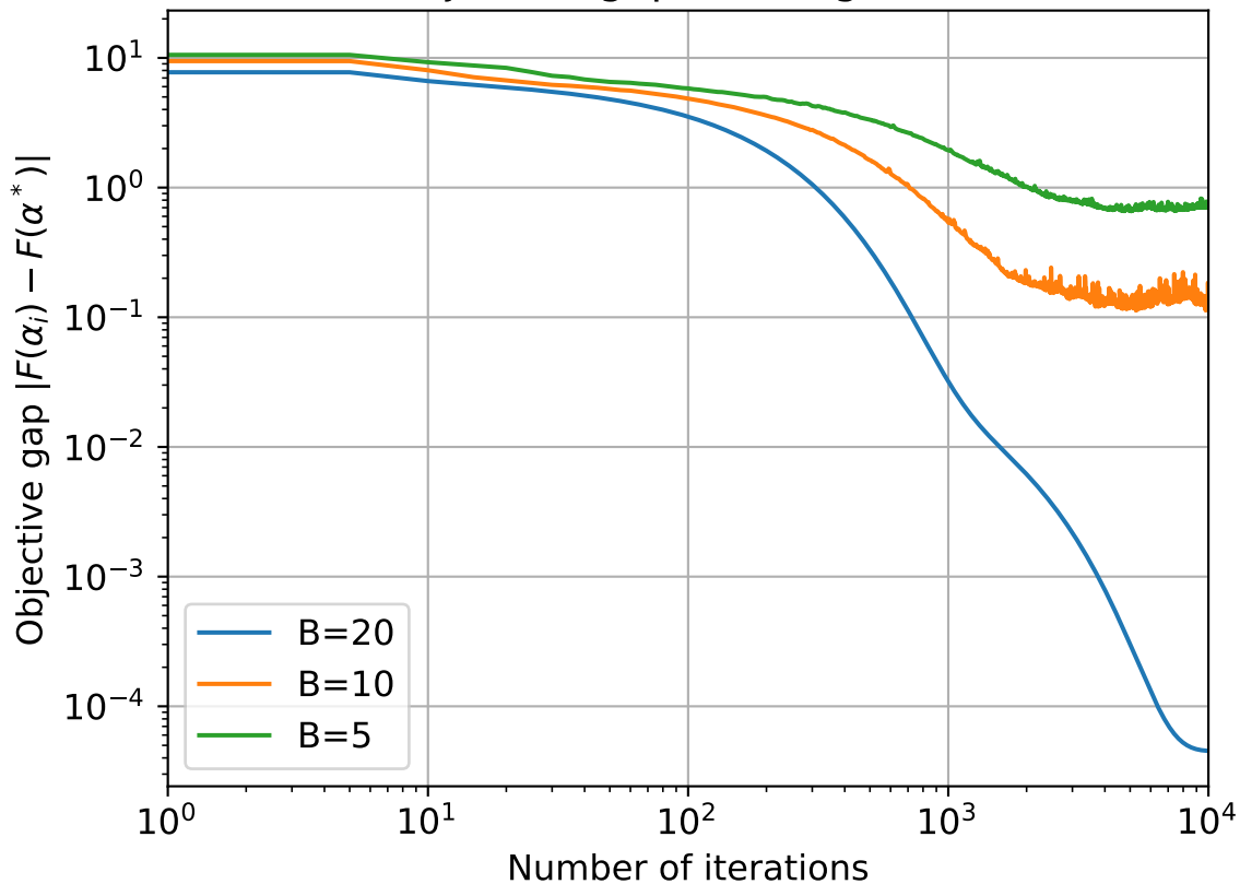
FedAVG : Objective gap convergence, E=5, C=5
