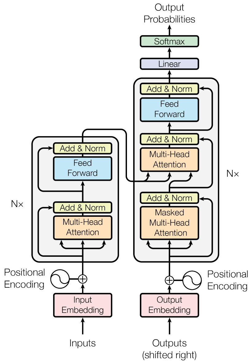
Figura 10.1: The architecture of the Transformer model.
