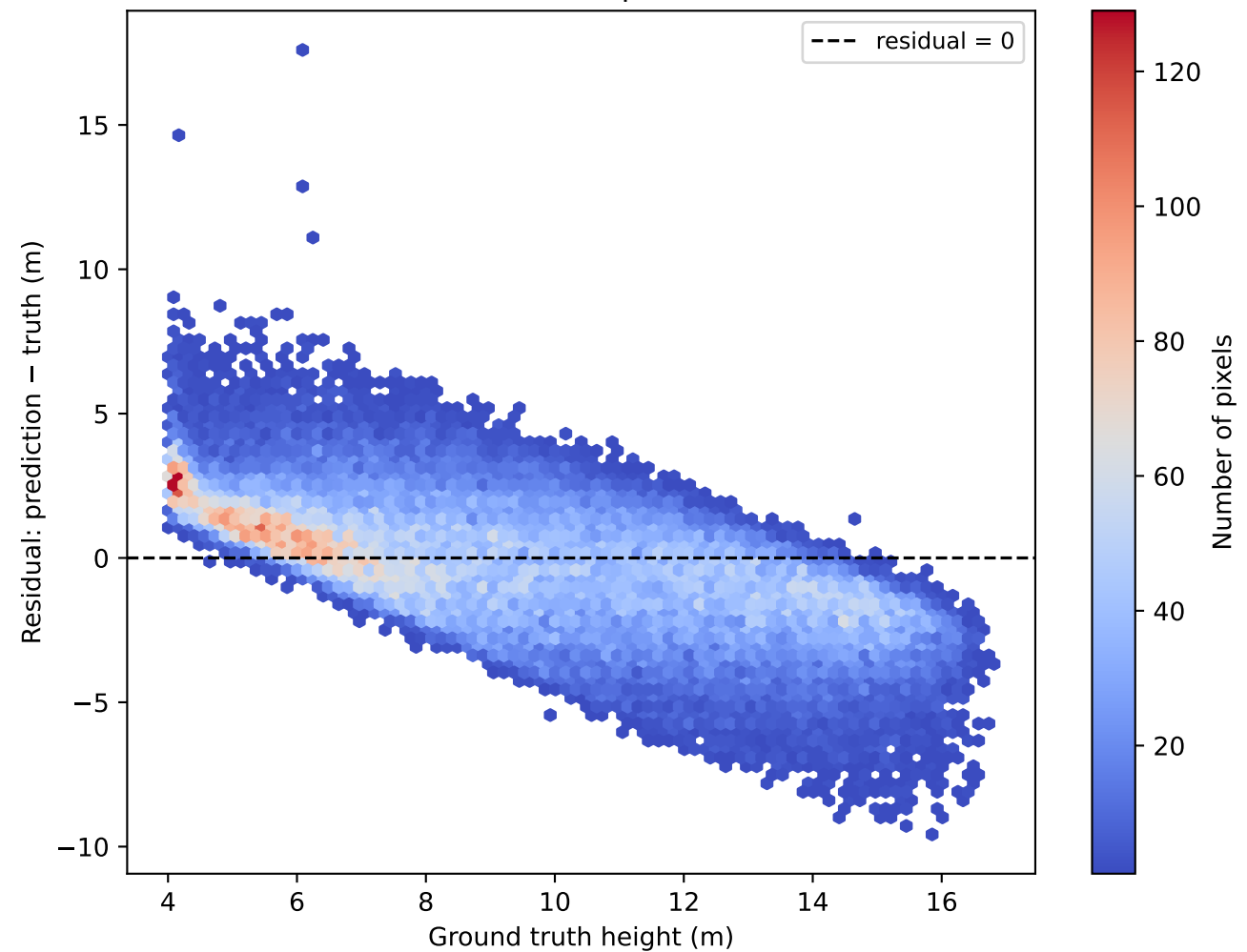
Residual plot
