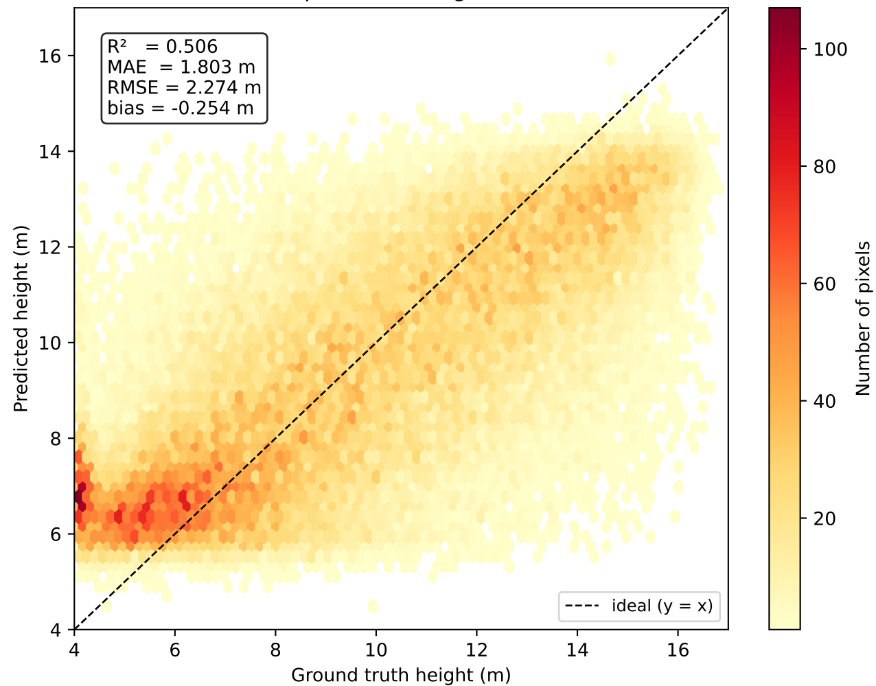
Scatter: prediction vs ground truth
