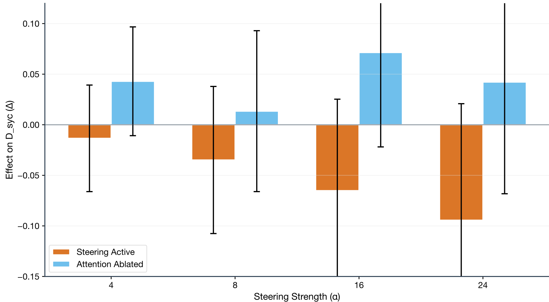
CAA Steering Effects by Alpha
