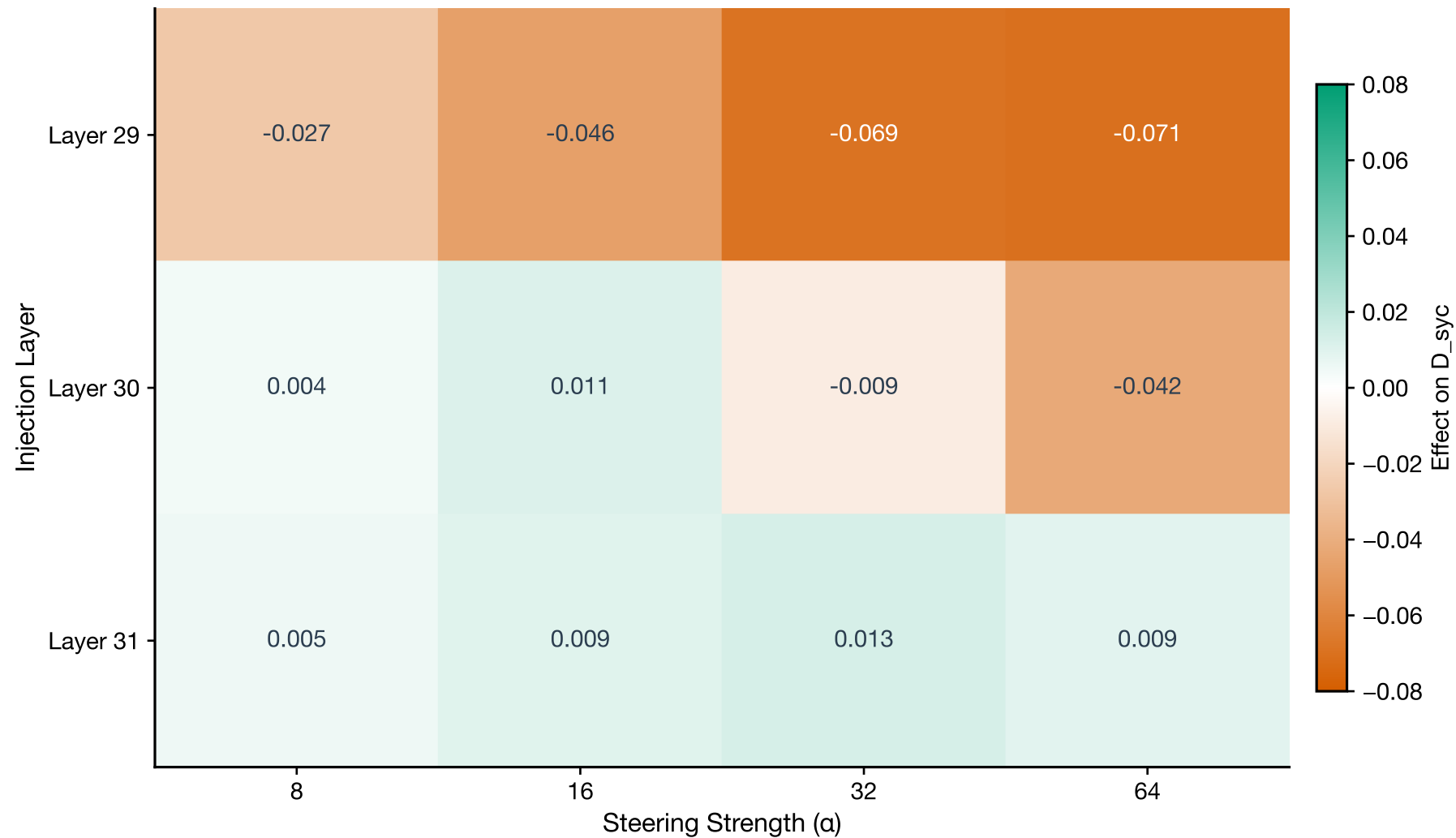
Late-Layer CAA Injection Effects
