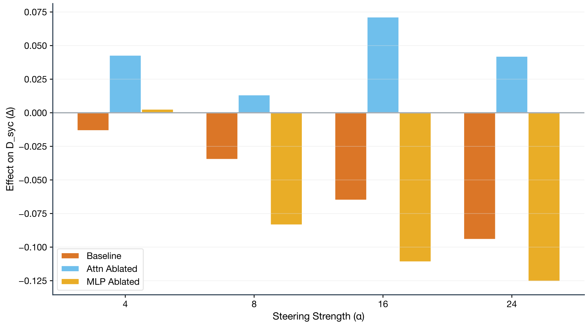
Steering Effects by Condition
