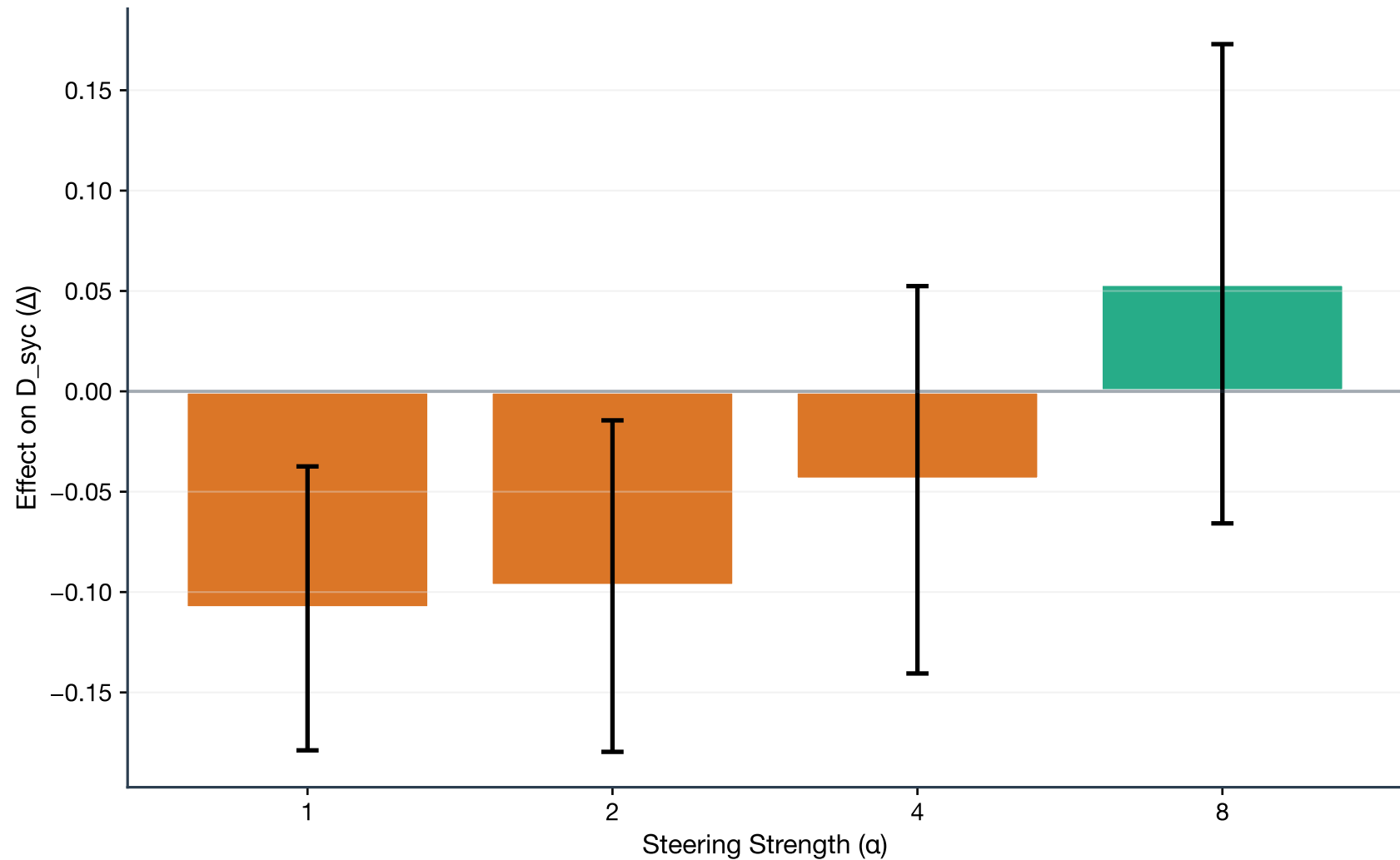
CCM Mean-Diff Steering Results
