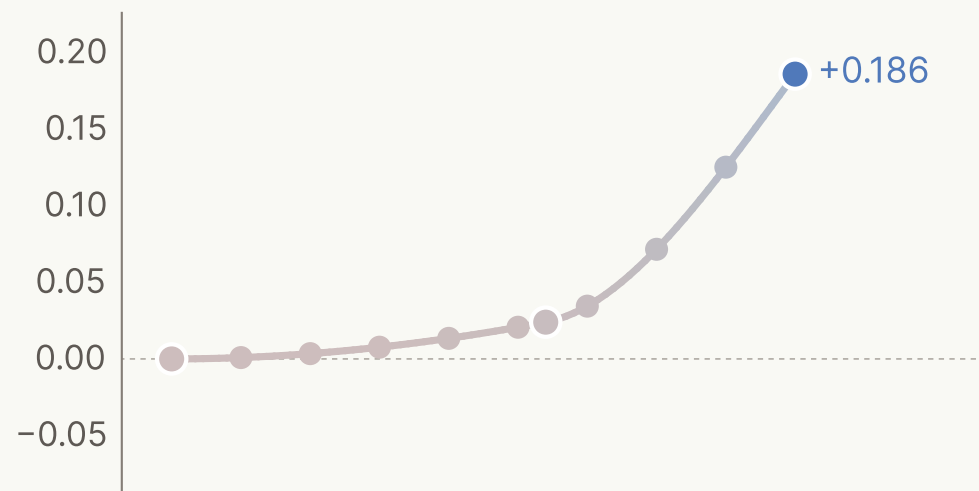
Qwen-3.5
