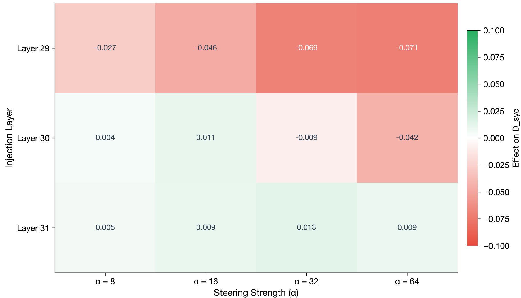
Late-Layer CAA Injection: No Consistent Effect
